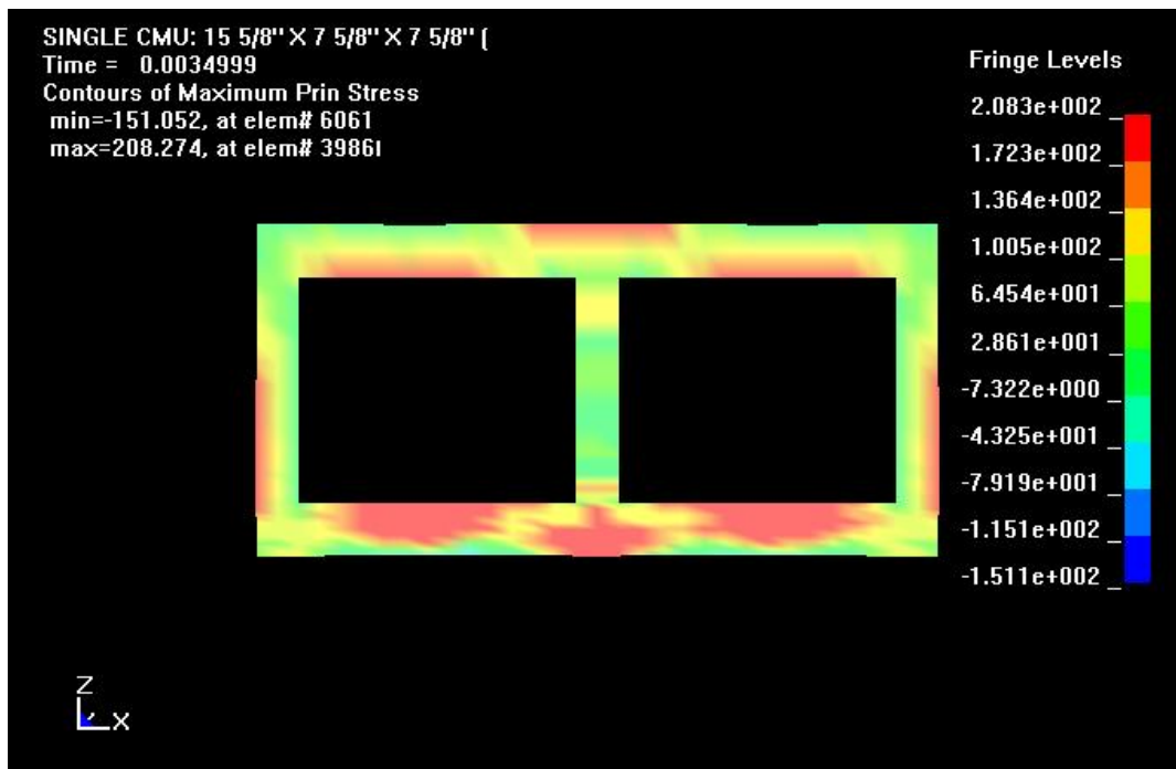
Figure 5.4-5 MAT_WINFRITH_CONCRETE Stress Fringes for 500 lb ANFO at 20 ft
