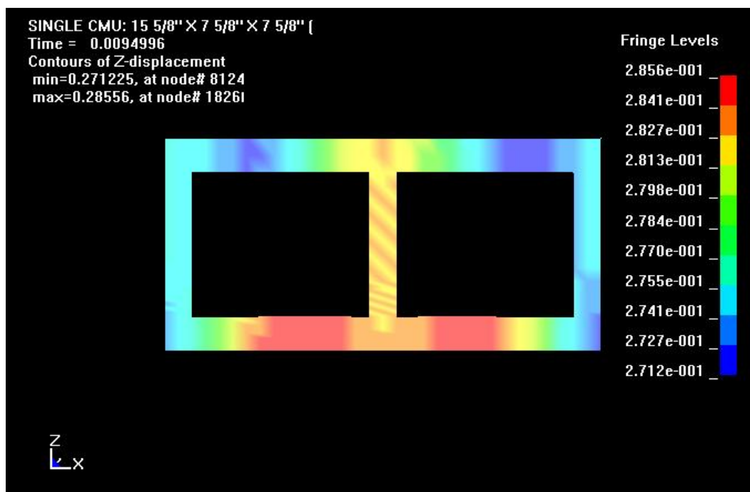
Figure 5.4-10 MAT_WINFRITH_CONCRETE Displacement Fringes for 500 lb ANFO at 30 ft
