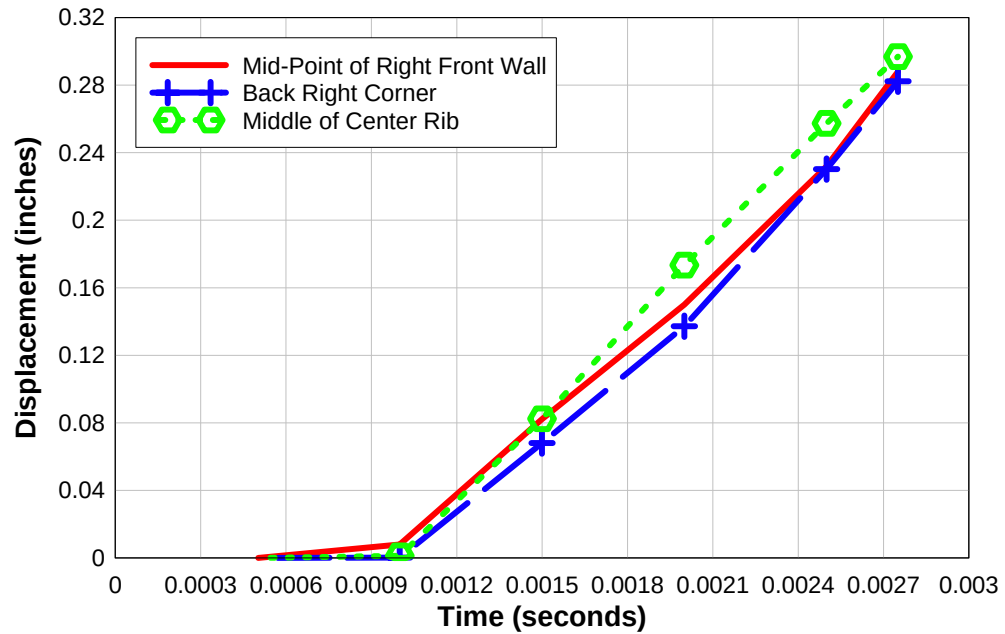
Figure 5.2-3 Displacement History Plots
