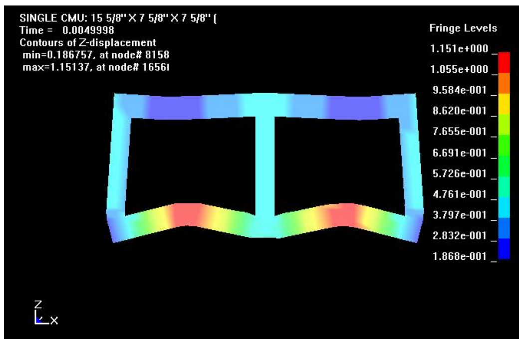
Figure 5.3-14 MAT_PSEUDO_TENSOR Displacement Fringes for 1000 lb ANFO at 20 ft
