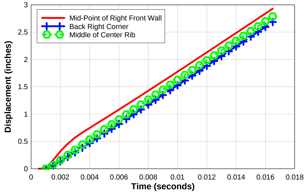
Figure 5.4-3 Displacement History Plots
