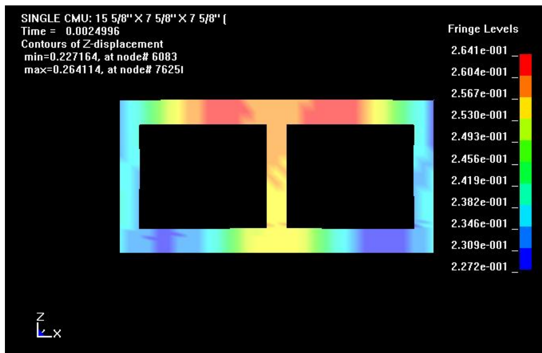
Figure 5.2-2 MAT_BRITTLE_DAMAGE Displacement Fringes for 500 lb ANFO at 10 ft
