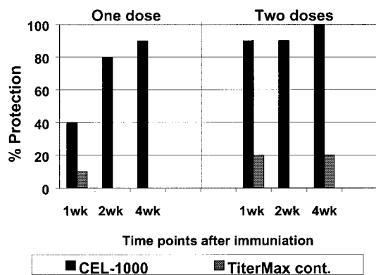
FIG. 4. Kinetics and duration of protection in A/J mice treated with CEL-1000 peptide before challenge. Mice ( n = 10 mice per group) that received one or two injections of 5 μg of CEL-1000 in TiterMax adjuvant at 3-week intervals and mice that received TiterMax adjuvant alone were challenged with 100 P. yoelii sporozoites at 1, 2, or 4 weeks after the last injection, followed by determination of parasitemia levels, as described in Materials and Methods. Protection was defined as negative blood smear results through 14 days postchallenge.
