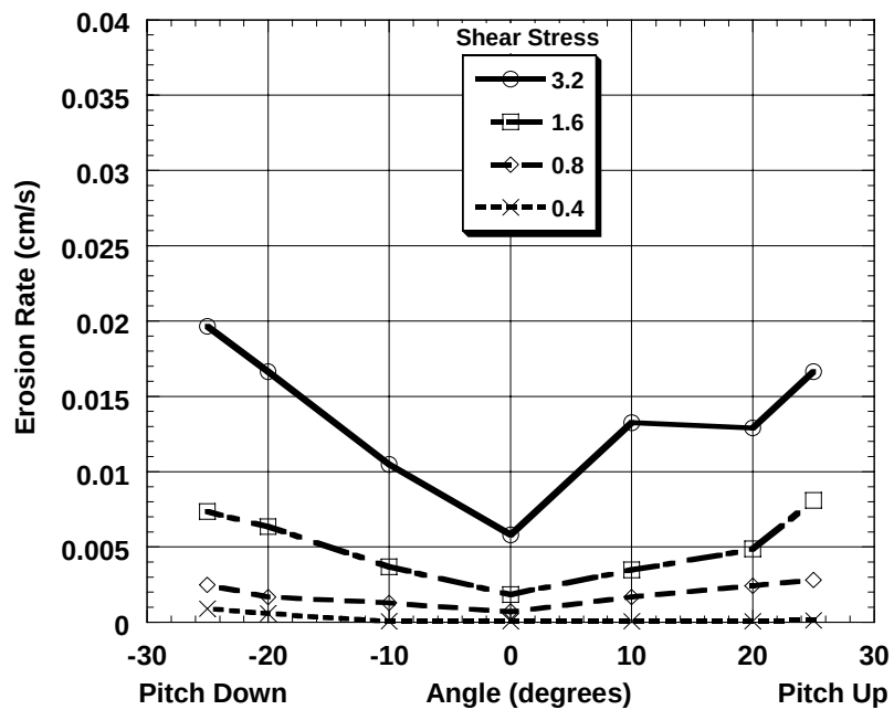
Figure 4.2e: Erosion Rate as a Function of Pitch Angle with Shear Stress ( \text{N/m}^2 ) as a Parameter for 5 \mu\text{m} Quartz. Consolidation time is 10 d.
