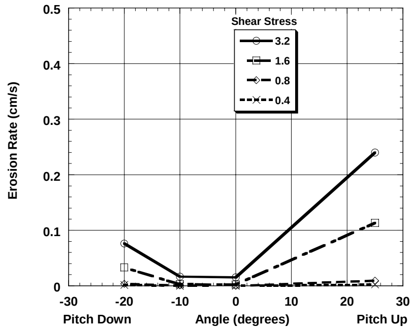
Figure 4.3: Erosion Rate as a Function of Pitch Angle with Shear Stress ( \text{N/m}^2 ) as a Parameter for 280 \mu\text{m} Quartz. Consolidation time is 64 d.
