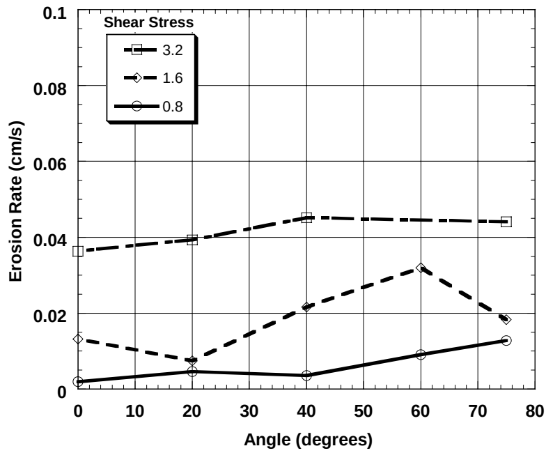
Figure 4.4f: Erosion Rate as a Function of Roll Angle with Shear Stress ( \text{N/m}^2 ) as a Parameter for 75 \mu\text{m} Quartz
