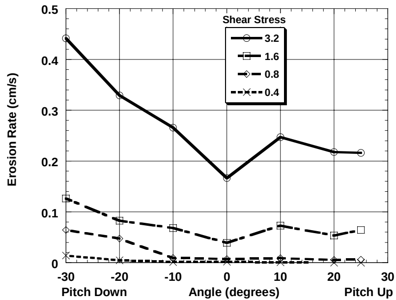
Figure 4.1b: Erosion Rate as a Function of Pitch Angle with Shear Stress ( \text{N/m}^2 ) as a Parameter for 280 \mu\text{m} Quartz. Consolidation time is 3 d.
