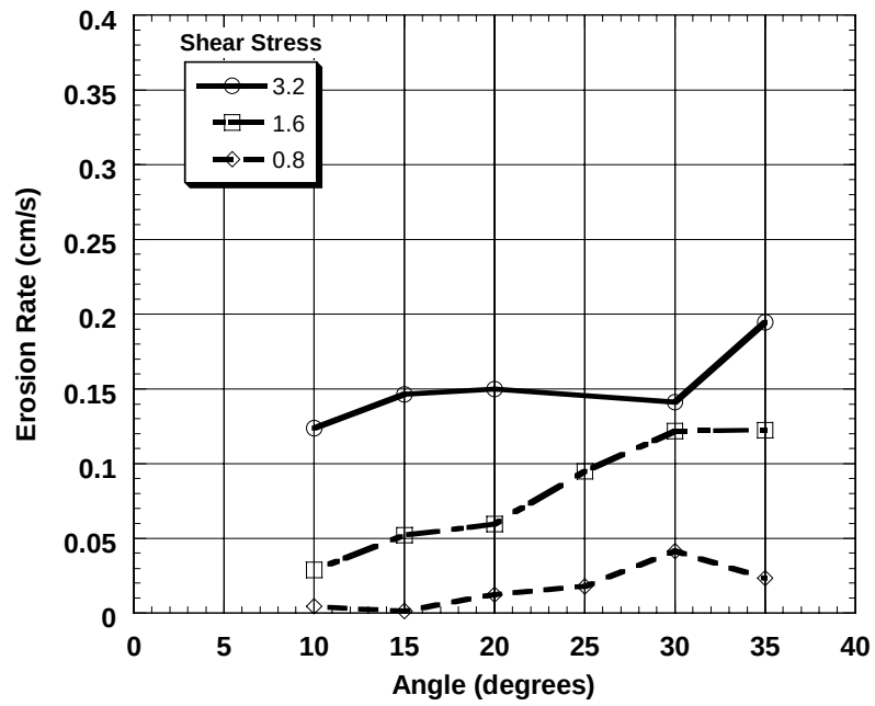
Figure 4.4d: Erosion Rate as a Function of Roll Angle with Shear Stress ( \text{N/m}^2 ) as a Parameter for 140 \mu\text{m} Quartz
