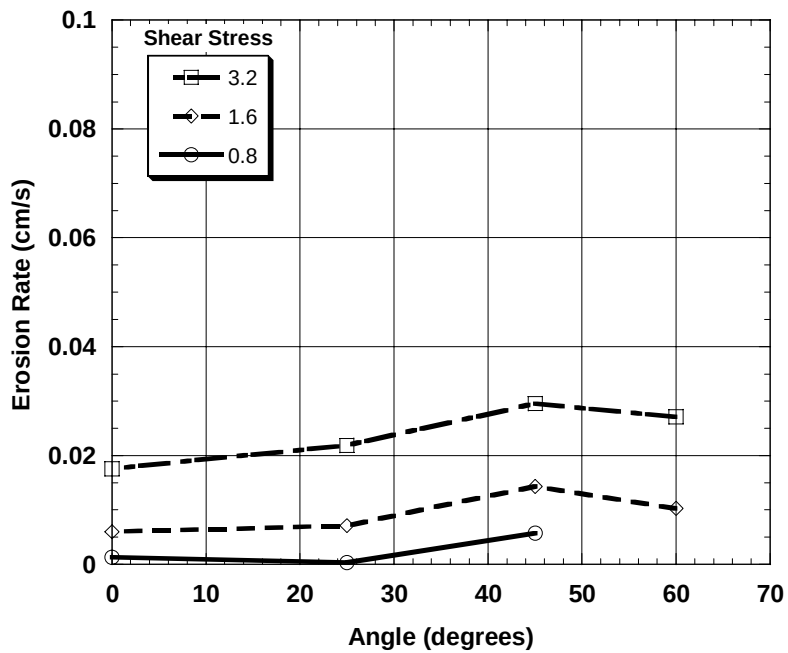
Figure 4.4g: Erosion Rate as a Function of Roll Angle with Shear Stress ( \text{N/m}^2 ) as a Parameter for 48 \mu\text{m} Quartz
