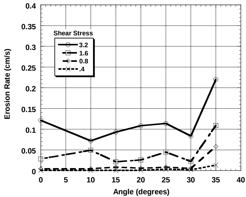
Figure 4.4c: Erosion Rate as a Function of Roll Angle with Shear Stress ( \text{N/m}^2 ) as a Parameter for 160 \mu\text{m} Quartz
