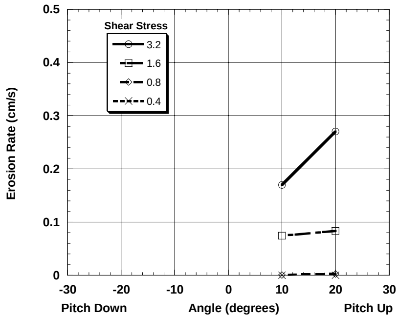
Figure 4.2a: Erosion Rate as a Function of Pitch Angle with Shear Stress ( \text{N/m}^2 ) as a Parameter for 1350 \mu\text{m} Quartz. Consolidation time is 10 d.
