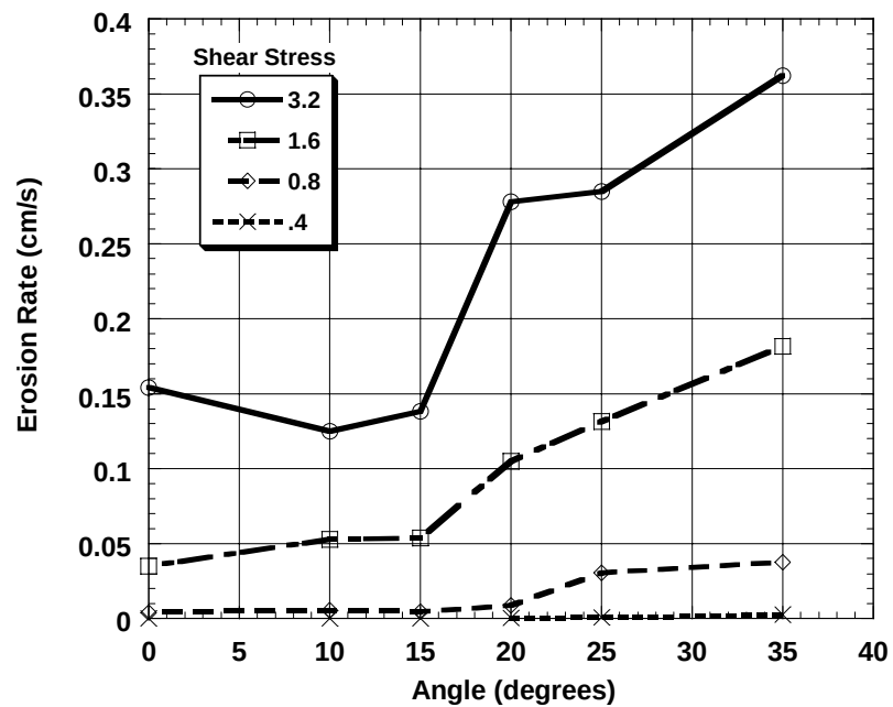
Figure 4.4a: Erosion Rate as a Function of Roll Angle with Shear Stress ( \text{N/m}^2 ) as a Parameter for 1350 \mu\text{m} Quartz.
