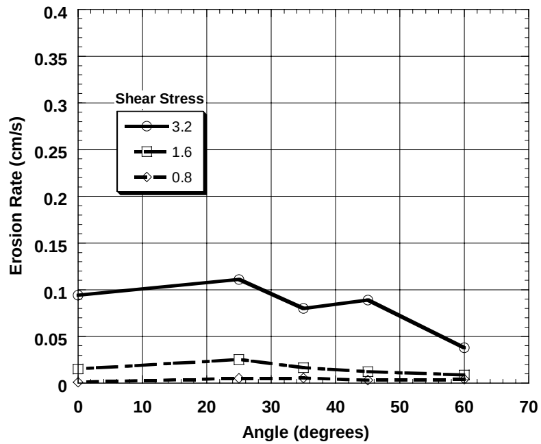
Figure 4.6 Erosion Rate as a Function of Roll Angle with Shear Stress ( \text{N/m}^2 ) as a Parameter for 160 \mu\text{m} Quartz with 5.0 % 20 \mu\text{m} Quartz Added.
