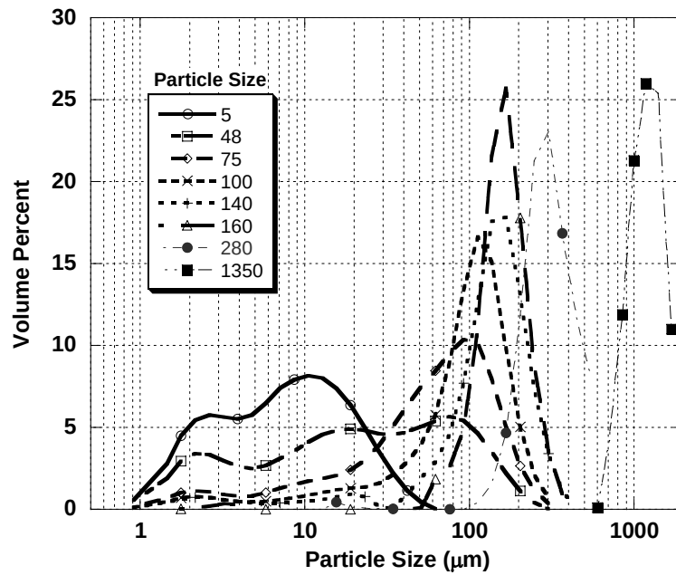
Figure 3.3: Particle Size Distributions of 5, 48, 75, 100, 140, 160, 280, and 1350 \mu\text{m} Quartz.
