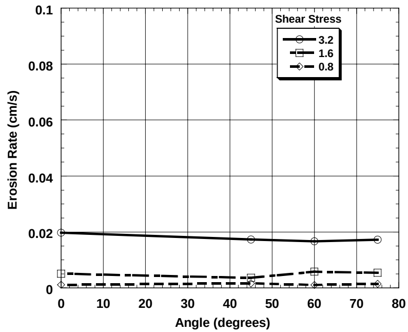
Figure 4.4h: Erosion Rate as a Function of Roll Angle with Shear Stress ( \text{N/m}^2 ) as a Parameter for 5 \mu\text{m} Quartz
