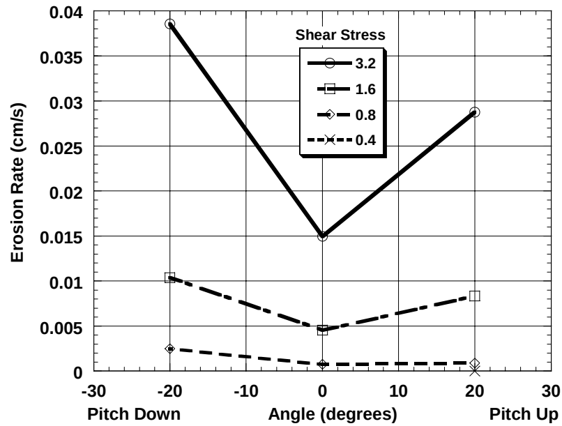
Figure 4.1e: Erosion Rate as a Function of Pitch Angle with Shear Stress ( \text{N/m}^2 ) as a Parameter for 5 \mu\text{m} Quartz. Consolidation time is 3 d.
