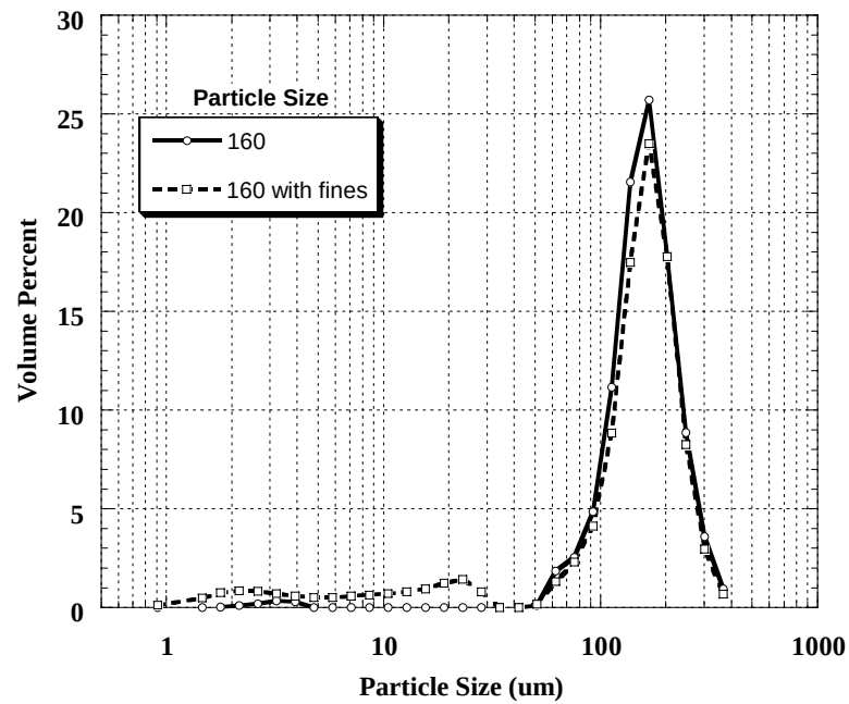
Figure 4.5: Particle Size Distribution for 160 \mu\text{m} Quartz with Added 5.0% 20 \mu\text{m} Quartz.
