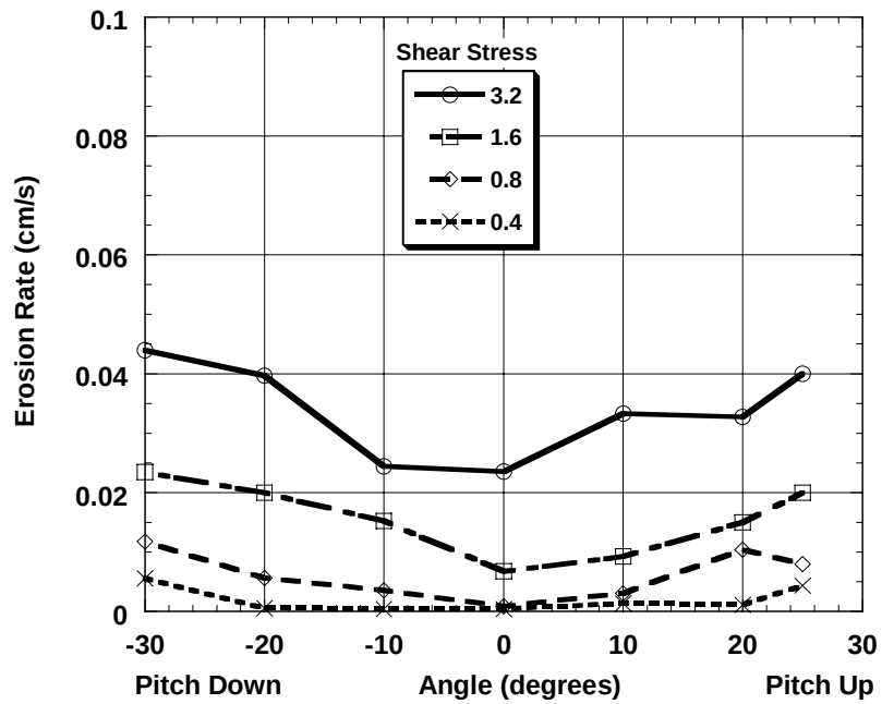
Figure 4.2d: Erosion Rate as a Function of Pitch Angle with Shear Stress ( \text{N/m}^2 ) as a Parameter for 48 \mu\text{m} Quartz. Consolidation time is 10 d.
