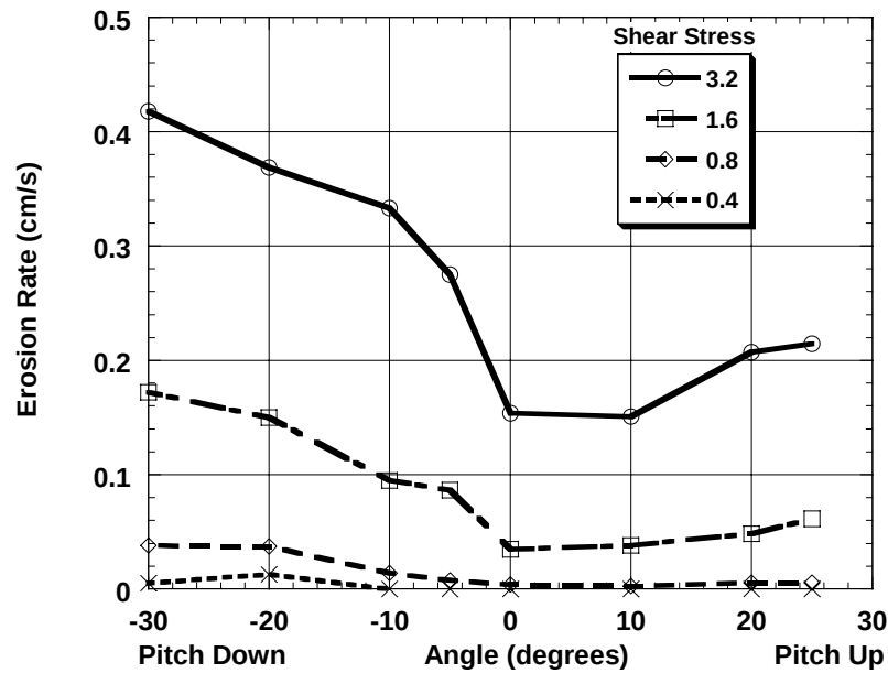
Figure 4.1a: Erosion Rate as a Function of Pitch Angle with Shear Stress ( \text{N/m}^2 ) as a Parameter for 1350 \mu\text{m} Quartz. Consolidation time is 3 d.
