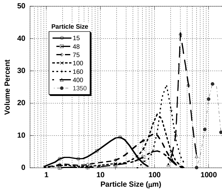
Figure 4.7: Particle Size Distributions of 15, 48, 75, 100, 160, 400 and 1350 \mu\text{m} Quartz.
