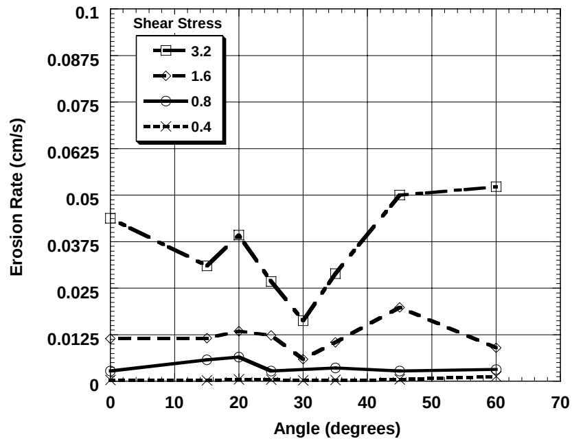
Figure 4.4e: Erosion Rate as a Function of Roll Angle with Shear Stress ( \text{N/m}^2 ) as a Parameter for 100 \mu\text{m} Quartz
