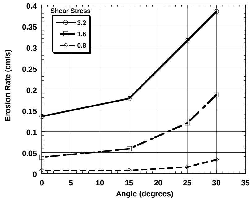
Figure 4.4b: Erosion Rate as a Function of Roll Angle with Shear Stress ( \text{N/m}^2 ) as a Parameter for 280 \mu\text{m} Quartz.
