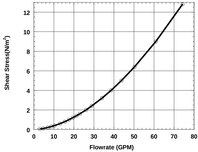
Figure 3.2: Shear Stress( \text{N/m}^2 ) as a Function of Flowrate (GPM) for Sedflume
