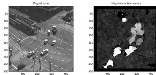
Figure 30: Optical flow applied to image sequence with camera pan. The background regions now contain noise due to the camera panning motion
