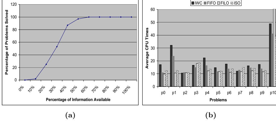
Fig. 4. Chart (a) shows the percentage of times ENQUIRER could find plans for the Delivery problems, as a function of the amount of information available during planning. Chart (b) shows the comparison of the average CPU times (in secs.) of the four query-processing strategies in ENQUIRER.
