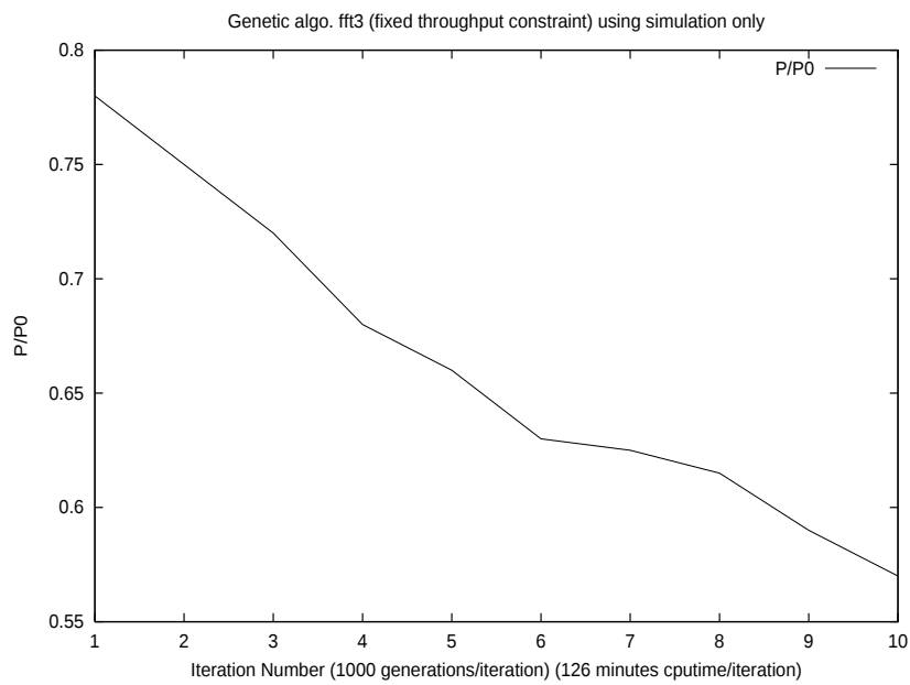
Figure 6. Plot of (\text{optimized power})/(\text{initial power}) vs. genetic algorithm iteration using simulation only.
