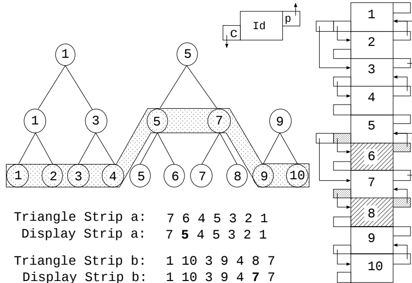
Figure 14: Skip Strip for Triangle Mesh in Figure 12 after two edge collapses
