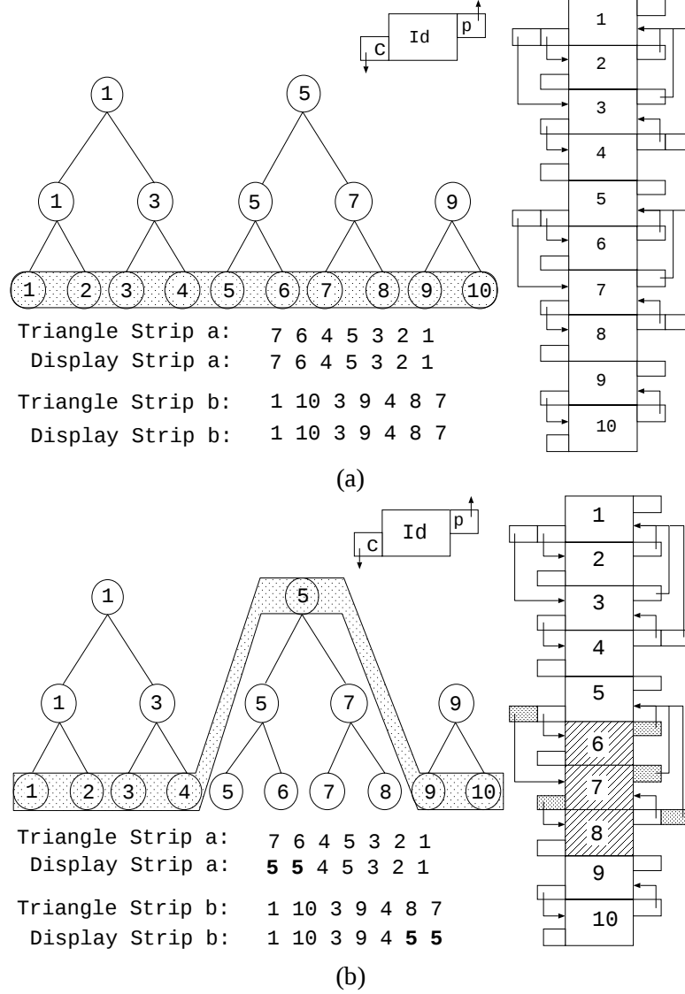
Figure 15: More efficient Skip Strip representations for Figures 13 and 14
