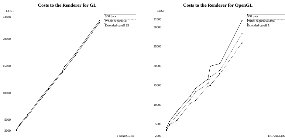
Figure 16: Overall cost comparisons for GL and OpenGL cost models.
