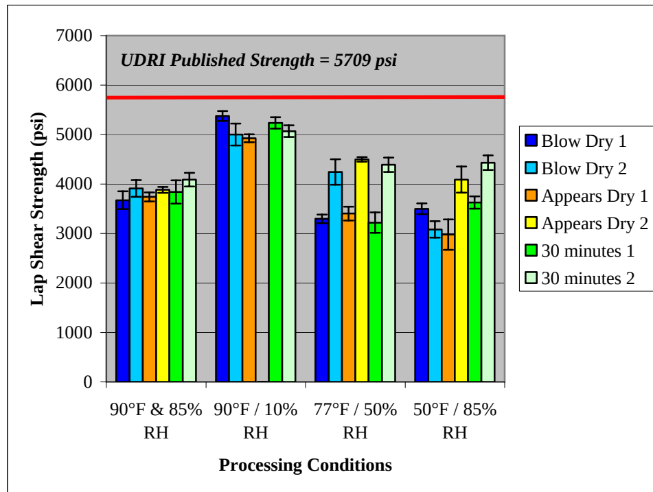
Figure 7: Lap Shear Strength Versus Processing Conditions for NP/SG with Fused BR 6747-1 Cocured with EA 9696 Adhesive
