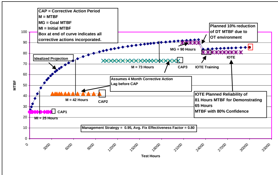
Figure 12. PM2 Reliability Growth Planning Curve.
