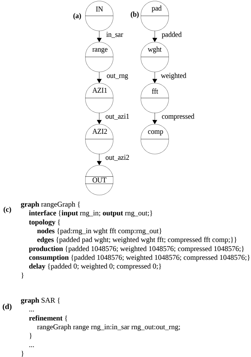
Figure 3. (a) The top-level partitioned application graph of a SAR application in the MCCI Autocoding Toolset. (b) Range processing. (c) Range processing in DIF. (d) Range processing instantiation in SAR. Note that although 3(c) is a single rate graph, the Autocoding Toolset presently exports this in the more general form of a DIF graph. This example is adapted due to space constraints.
