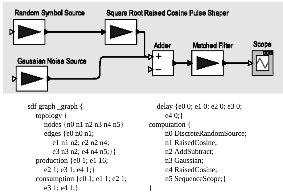
Figure 2. Ptolemy II model of a PAM communication system that is exported to DIF. This example represents the functionality of each node as a computation attribute, which is derived from the Ptolemy II library definition.
