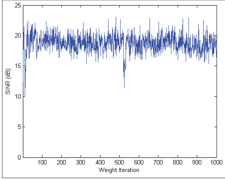
Figure 14. SINR in simulation trial for anticipative maximin algorithm with W_h = 30 MHz and two interference signals at 40^\circ and -10^\circ .
