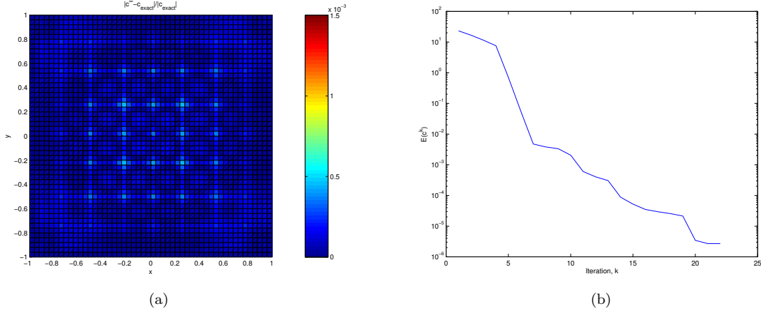
Figure 8: (Example 1. 98 Sources) 3-D case. (a): the relative error in the solution on the cross-section z = 1 and (b): the convergence history of energy.
