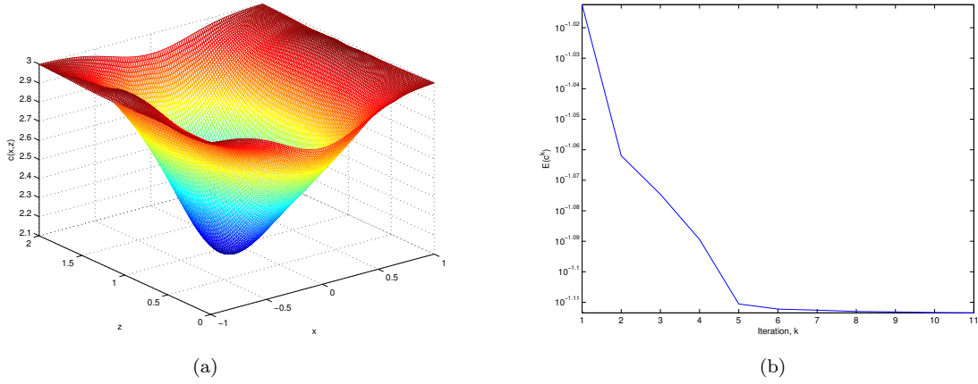
Figure 6: (Example 3 with added noise. Ten Sources) BFGS. (a): the final approximated c ; (b): the convergence history of energy.
