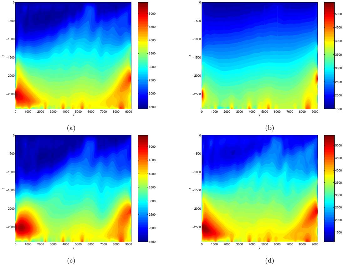
Figure 11: (Marmousi model) Converged solutions. (a): \nu = 10^4 and \Delta x = 24 ; (b): \nu = 10^2 and \Delta x = 24 ; (c): \nu = 10^6 and \Delta x = 24 ; (d): \nu = 10^4 and \Delta x = 12 .
