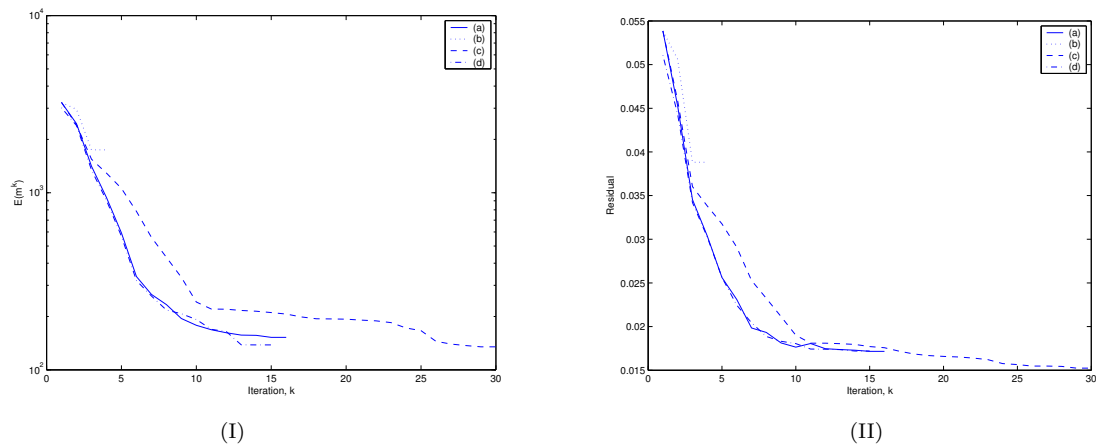
Figure 12: (Marmousi model) The change in (I): the energy and (II): the residual. Legend: (a): \nu = 10^4 and \Delta x = 24 ; (b): \nu = 10^2 and \Delta x = 24 ; (c): \nu = 10^6 and \Delta x = 24 ; (d): \nu = 10^4 and \Delta x = 12 .
