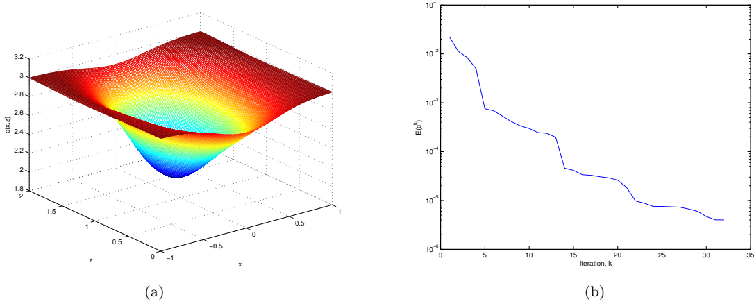
Figure 4: (Example 3. Ten Sources) BFGS. (a): the final approximated c and (b): the convergence history of energy.
