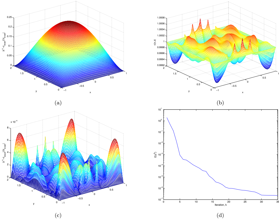
Figure 1: (Example 1. Ten Sources) BFGS. (a): the initial guess; (b): final approximated c ; (c): the relative error in the solution; (d): the convergence history of energy.
