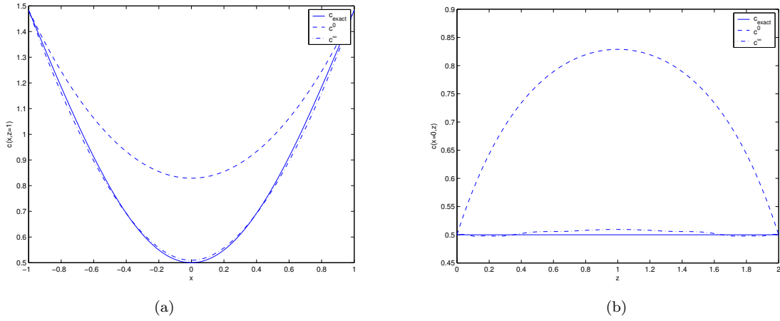
Figure 3: (Example 2. Ten Sources) Cross-sections of the solutions. (a): z = 1 and (b): x = 0 .
