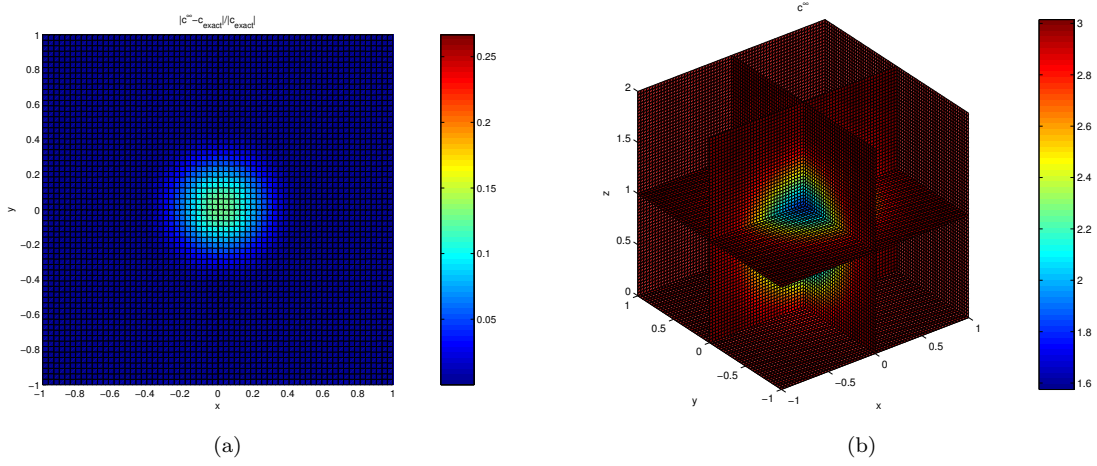
Figure 9: (Example 2. 98 Sources) 3-D case. (a): the relative error in the solution on the cross-section z = 1 and (b): the final approximated c .
