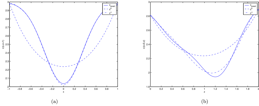
Figure 5: (Example 3. Ten Sources) BFGS. Cross-sections of the solutions. (a): z = 1 and (b): x = 0 .
