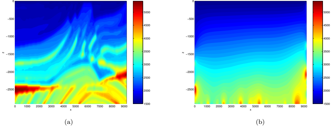
Figure 10: (Marmousi model) (a): the true velocity distribution and (b): the initial profile c^0 .
