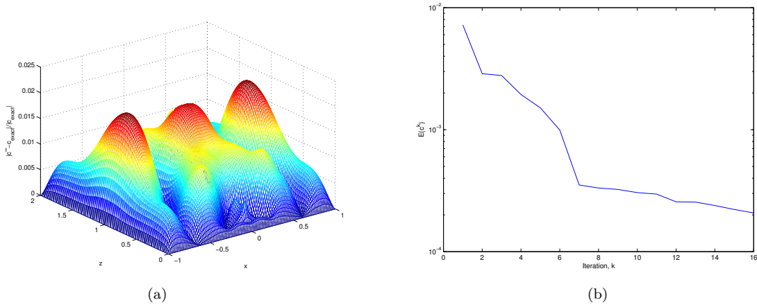
Figure 2: (Example 2. Ten Sources) (a): the relative error in the solution and (b): the convergence history of energy.
