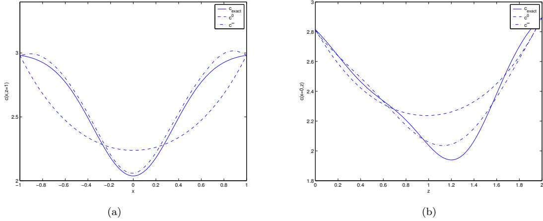
Figure 7: (Example 3 with added noise. Ten Sources) BFGS. Cross-sections of the solutions: (a): z = 1 and (b): x = 0 .
