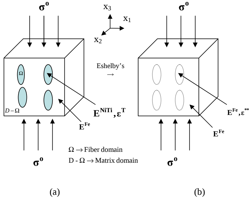
Figure 7. Eshelby's Inhomogeneity Inclusion problem for use in the simulation of the second stage behavior of SS curve of a SMA composite.
