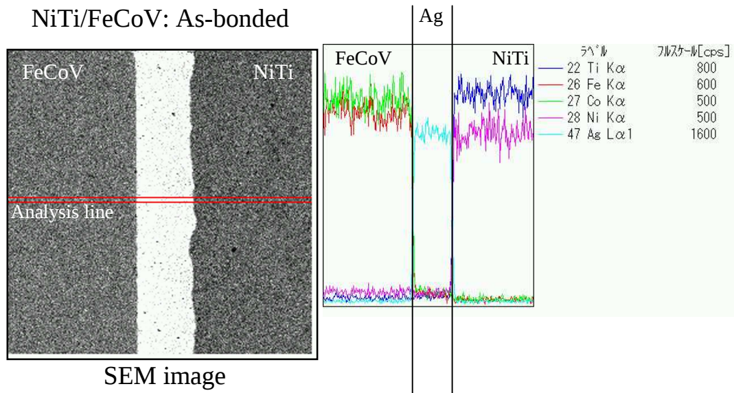
(c) EDX analysis of NiTi/FeCoV Sheet Composite, There are no inclusions, compounds at interface.
