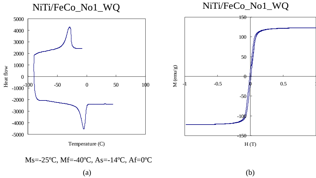
Figure 33. (a) DSC data, (b) M-H curve of TiNi/FeCoV composite.
