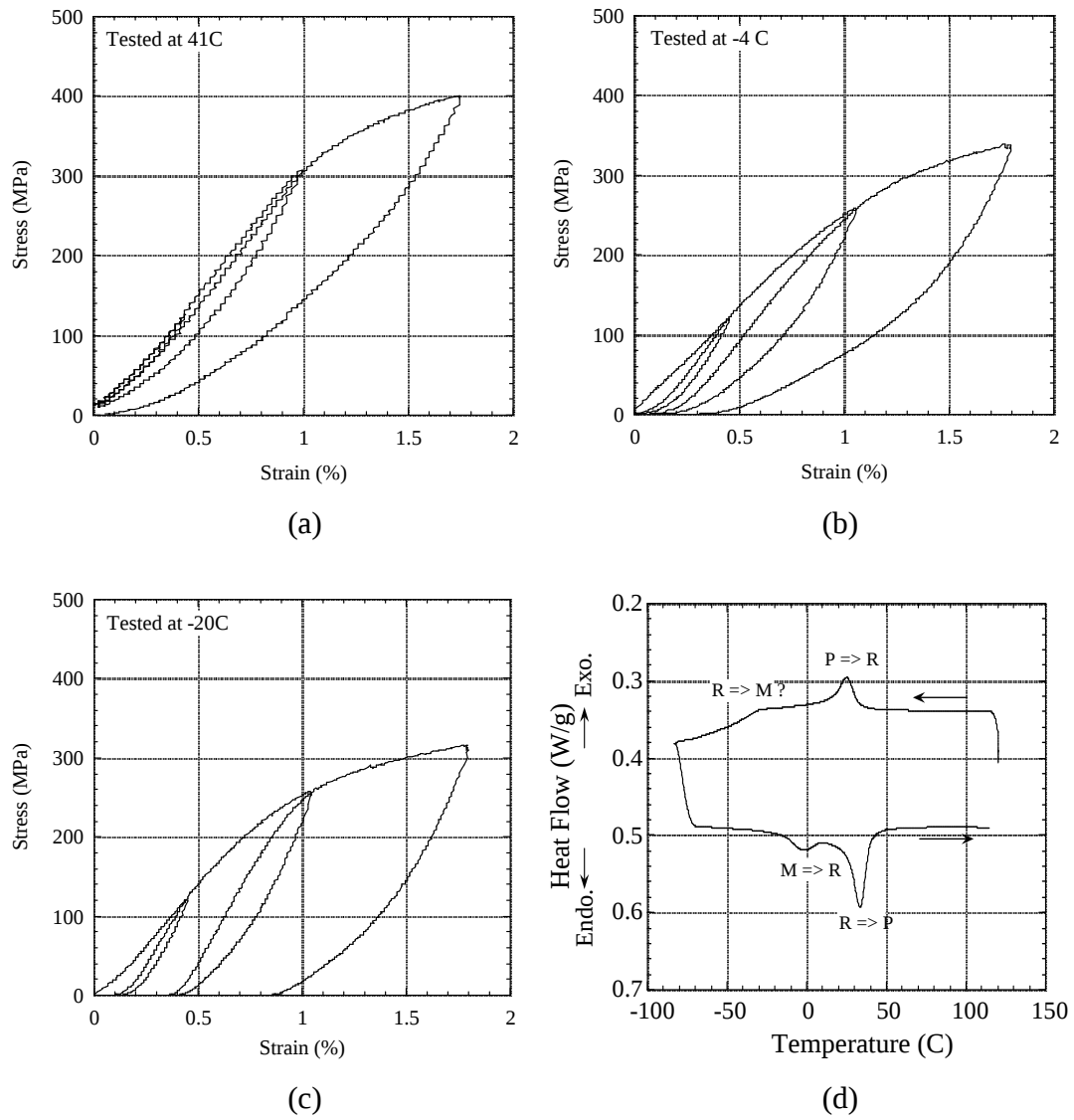
Figure 29. Changes in S-S Curve at Various Temperatures in TiNi / Fe Composite
