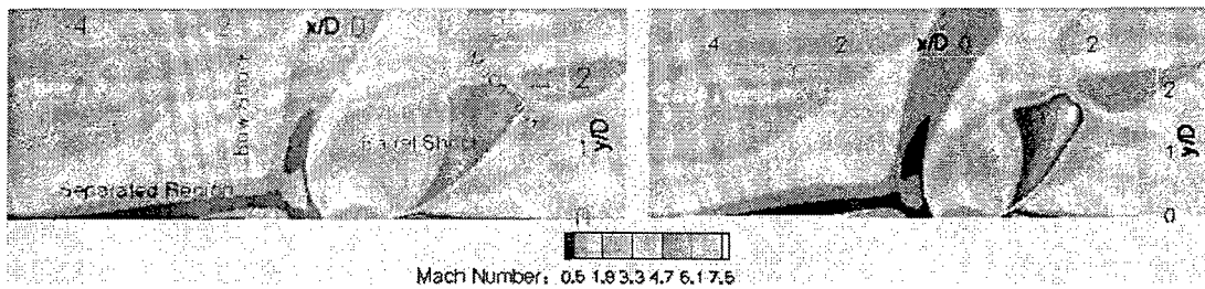
Figure 13: Jet in crossflow: Mach number contours in the x - y plane at the centerline ( z = 0 , or plane of symmetry) for two injected fluids (air, left, and helium, right). Shock structures and upstream recirculating region are identified.
