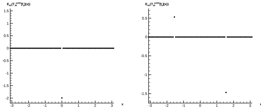
Figure 3.8: Application of (3.22) ( \tilde{E}_{80}^\tau[f](x) ) to approximate (a) [f_a](x) and (b) [f_b](x) .
