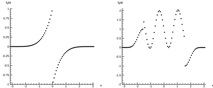
Figure 2.1: (a) [f_a](x) and (b) [f_b](x) on N = 80 equally spaced grid points.
