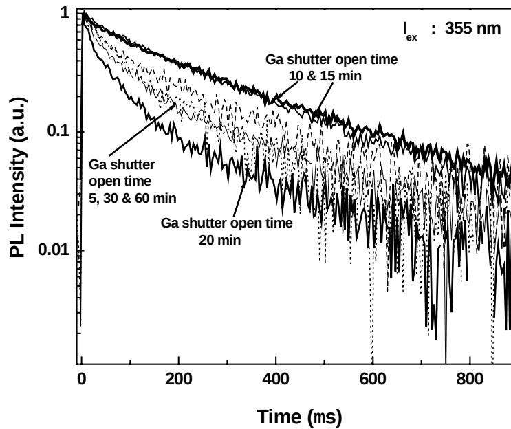
Figure 2. PL decay transients of GaN:Eu films under above-gap excitation (355 nm) at 300 K.
