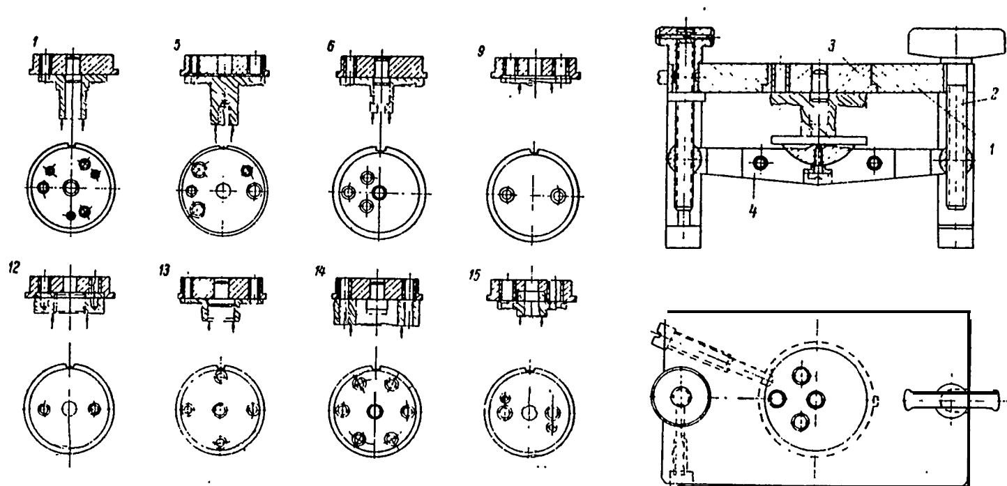
Figure 10, Example of a group drill jig and adapters used for drilling 8 different parts in a part family
