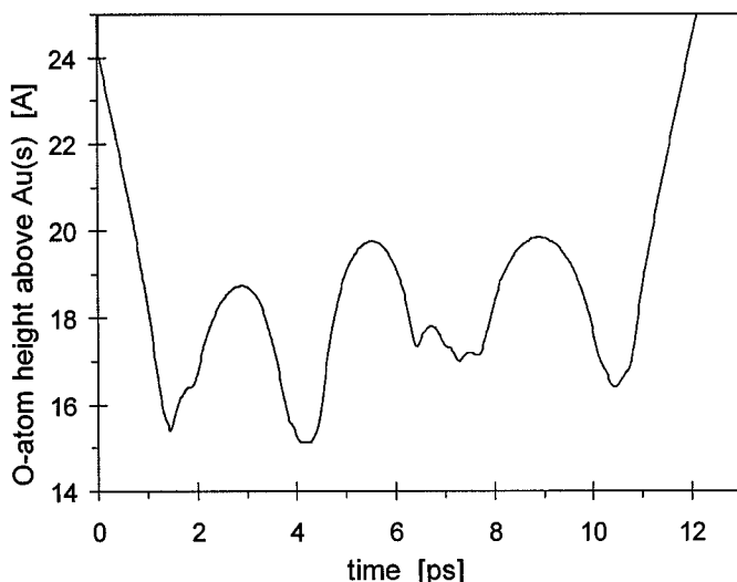
Figure 11. Plot of the oxygen atom height above Au(s) for a selected trajectory with multiple hops. The terminal methyl groups are located at ~14.6 Å. This oxygen atom remains near the surface top at all times.
