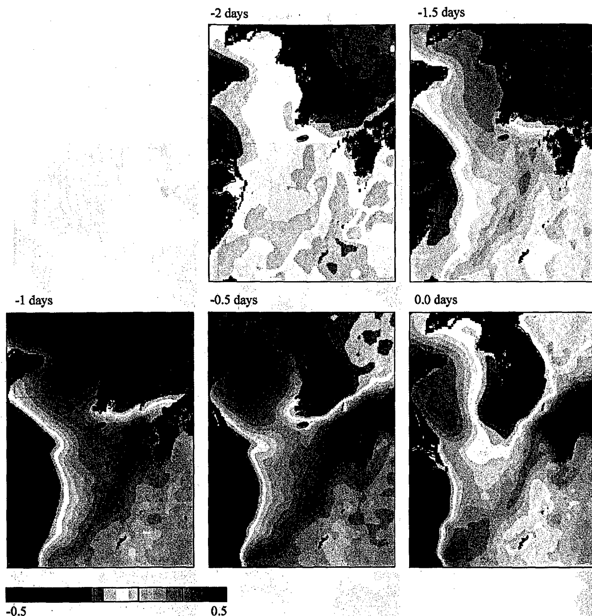
Plate 3. The lagged correlation between the numerical model sea level and the transport through the strait is indicated by the color. The area of greatest correlation propagates from the east Korea coast to the south Korea coast. This propagation is in line with dynamics of Kelvin waves or shelf waves. The sea-level change across the Korea Strait is expected to generate an increased geostrophic transport. A sea-level increase is also present along the shelf break of the East China Sea, which is in the region of wind sensitivity indicated by the adjoint model (Plate 4).
