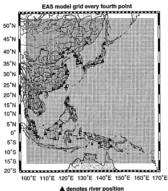
Fig. 1. The East Asian Seas NCOM model that provides the transport variations for this study is embedded within a large-domain model that provides boundary condition transport, temperature, and salinity.
