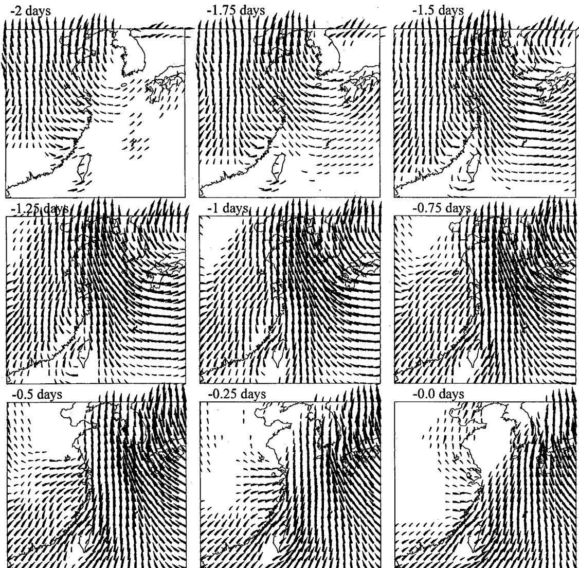
Fig. 4. The same as Fig. 3, but the cross-covariance is between the modeled transport time series and the wind-stress field. The results are similar. Differences are that the significance levels are higher due to the absence of noise in the modeled transport time series. Also, inaccuracies in the wind field would not affect the modeled transport cross-covariance with wind stress as much as the observed transport cross-covariance with wind stress.
