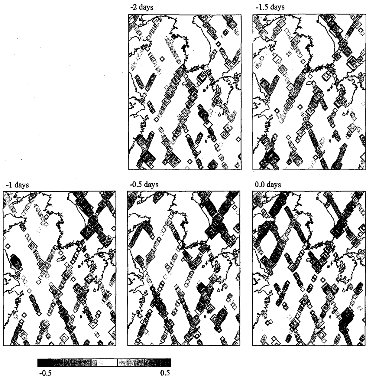
Plate 1. The lagged correlation between the sea level observed by the T/P satellite and the observed transport through the strait is indicated by the color. Correlations less than 1 standard deviation are not plotted. The symbol size indicates the confidence level, with small symbols being 1–2 standard deviations, medium-sized symbols 2–3 standard deviations, and large symbols greater than 3 standard deviations. The most significant correlation occurs at lags of –0.5 to –1.0 days (sea level precedes transport) off the east Korea coast with low sea level preceding transport increases.
