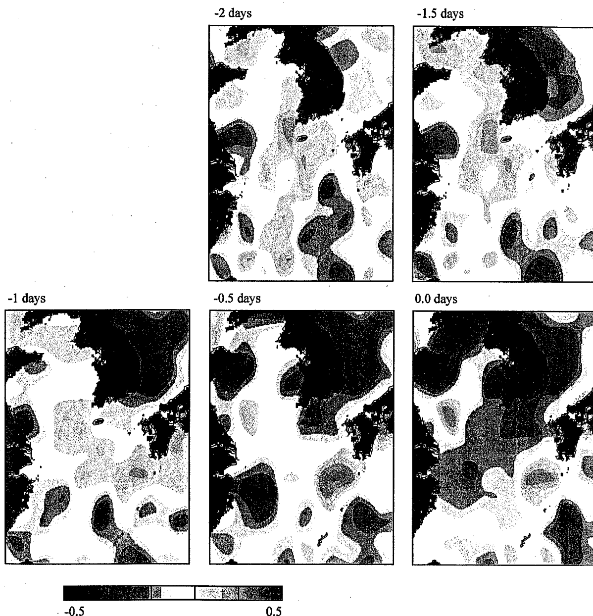
Plate 2. The lagged correlation between the sea level observed by the T/P satellite and the observed transport through the strait after a simple interpolation. The spatial sampling is coarse, but the interpolation aids in comparison with the model results (Plate 3).
