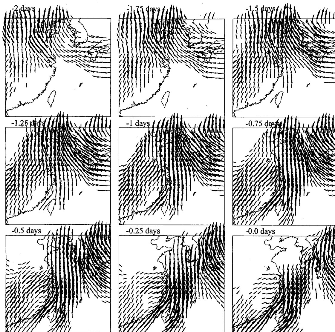
Fig. 3. The covariance of observed transport (Fig. 2) to wind stress is computed at each point in space. The vector components here represent the transport covariance to the zonal and meridional wind stress components at the specified lag. Increasing magnitude lag indicates that the wind variation precedes the transport variation. The line thickness indicates significance level. Covariances under 1 standard deviation of significance are not plotted, covariances up to 2 standard deviations are plotted with thin arrows, covariances from 2 to 3 standard deviations by medium arrows, and covariances above 3 standard deviations are plotted with thick arrows. The transport variations are mostly related to north-south wind stress variations across the Yellow, East China, and Japan/East Seas between -0.5 - and -1 -day lag (wind stress preceding the transport).
