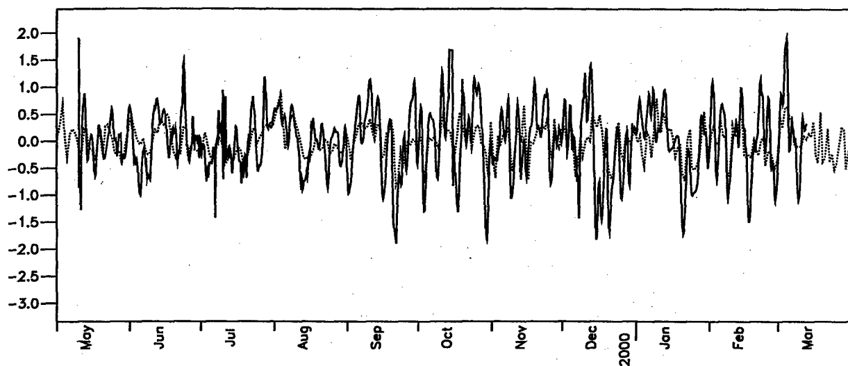
Fig. 2. The EAS numerical model (dashed) and observed transport (solid) through the Korea Strait are filtered to the synoptic band (2–20) days for direct comparison. Most of the transport events observed in the strait are reproduced in the model. These would be expected to be deterministically wind forced processes, and this indicates skill in the wind-forcing as well as the model dynamics.
