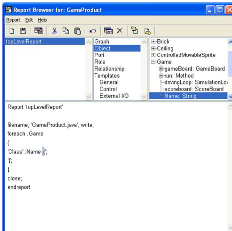
Figure 11: Report Browser
