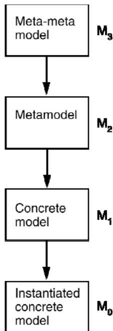
Figure 4: Meta-Tower for the MOF
