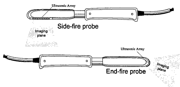
Fig. 4b: Schematic view of side-fire (top) and end-fire (bottom) transrectal probe for combined ultrasound, elasticity and strain-hardening imaging.
