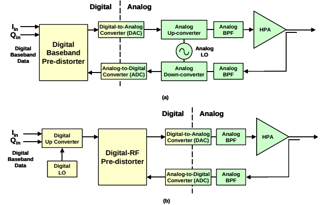
Fig. 5. (a) Digital baseband and (b) digital-RF predistortion schemes.
