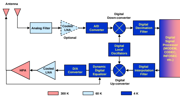
Fig. 1. Block diagram of conceptual digital-RF transceiver, where data conversion is carried out directly at RF frequencies, and signal extraction and processing are done using ultrafast superconducting digital electronic circuits (dark).
