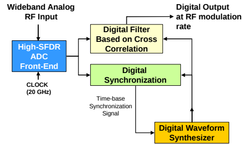
Fig. 5. The ADC front-end (modulator) produces a high-fidelity digitized RF waveform, which is correlated against the corresponding digital reference template waveform.
