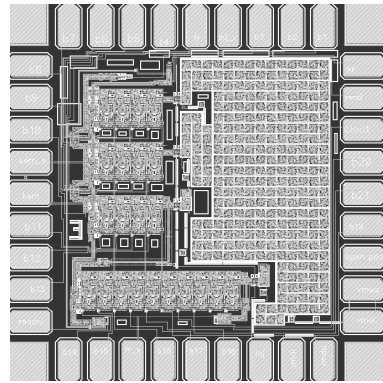
Fig. 8. An 18-bit RSFQ DAC chip. The 5 \times 5 mm 2 chip contains more than 2,000 Josephson junctions.
