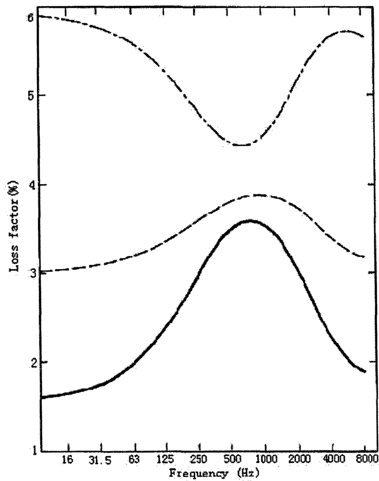
Figure 2.3. The frequency dependence of the damping in sandwich structures. Solid line, \eta_1 = 1.5\% , \eta_2 = 2\% ; dashed line, \eta_1 = 3\% , \eta_2 = 2\% ; dotted line, \eta_1 = 6\% , \eta_2 = 2\% .
