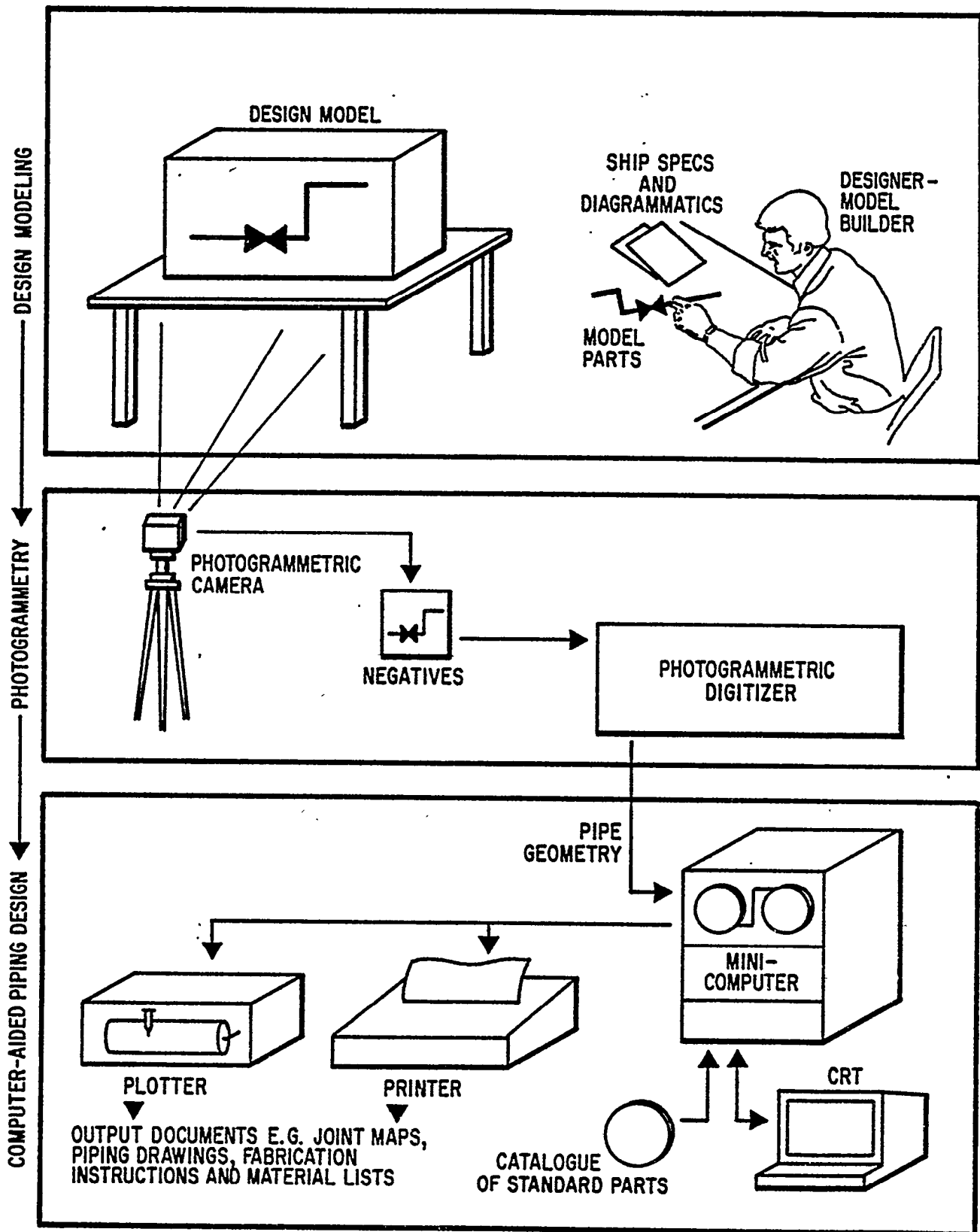
FIGURE 1.3 : The Marriage of Design Modeling, Photogrammetry and Computer-Aided Pipe Detailing Systems.
