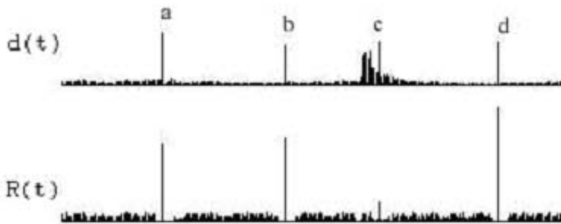
Figure 13: Effectiveness of second-max ratio criterion in detecting cuts. Note that the peaks due to motion that appear in d(t) do not appear in R(t)
