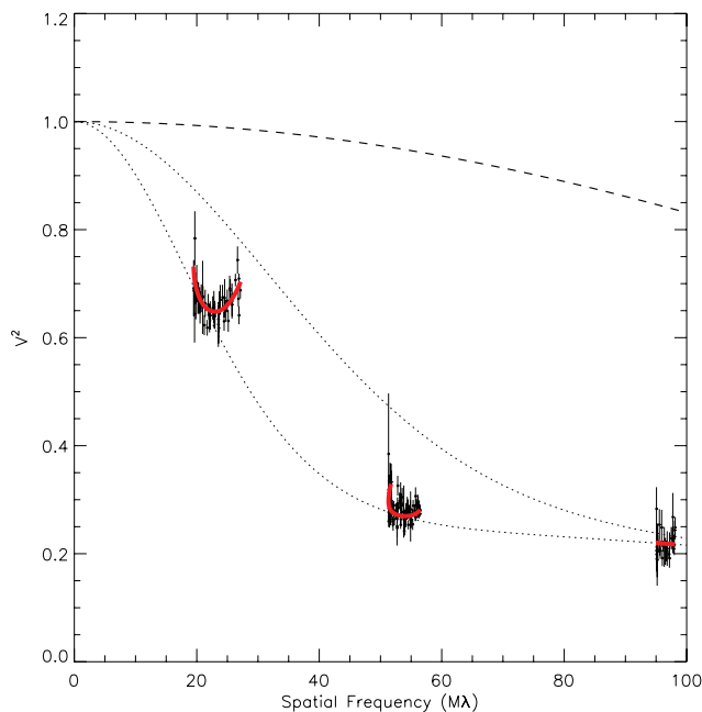
FIG. 7.—Calibrated squared visibilities from the H\alpha channel of \gamma Cas obtained at three baselines. The elliptical Gaussian model ( red solid line ) fitted to all observations is shown at each baseline for the same HA range as defined by the observations. The model contains a contribution from the stellar photospheric disk ( dashed line ) that is modeled with eq. (2). Model curves evaluated at the minor ( top dotted line ) and major ( bottom dotted line ) axes of the elliptical Gaussian model are also shown.
