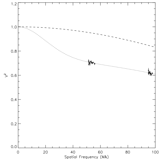
FIG. 9.—Calibrated squared visibilities from the H\alpha channel of \gamma Cas obtained on 2004 December 2 without the use of a narrowband filter at two baselines (AE-AW and AE-W7). The best-fit circularly symmetric Gaussian model ( dotted line ) and the stellar photospheric disk ( dashed line ) are also shown.
