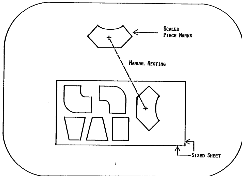
FIGURE 7 COMPUTER-AIDED NESTING
