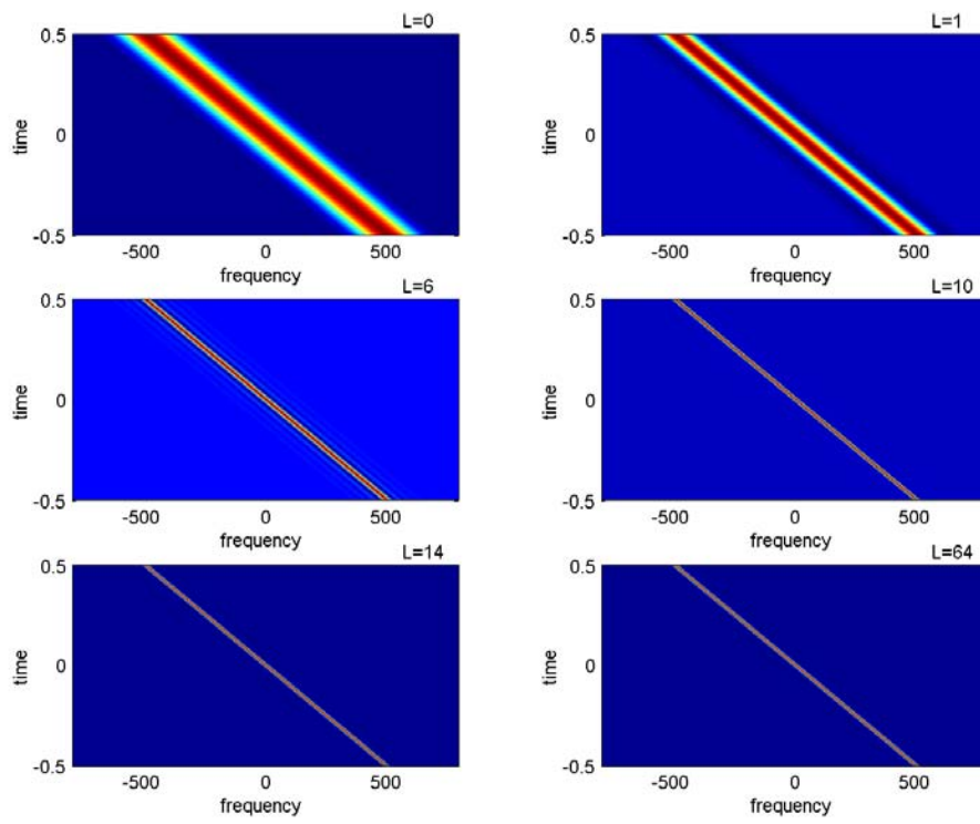
Figure 22: SM of a Linear Frequency Modulated Signal x(t) , with fixed window width N = 128 , and different L values
