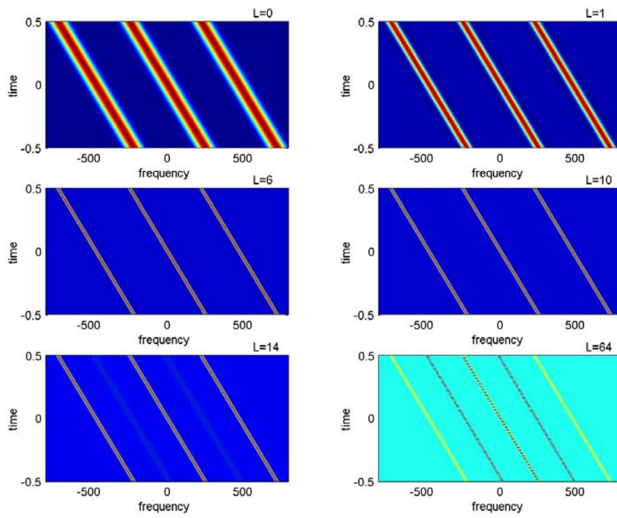
Figure 31: SM of three Linear Frequency Modulated Signal components x(t) , with fixed window width N = 128 , and different L values
