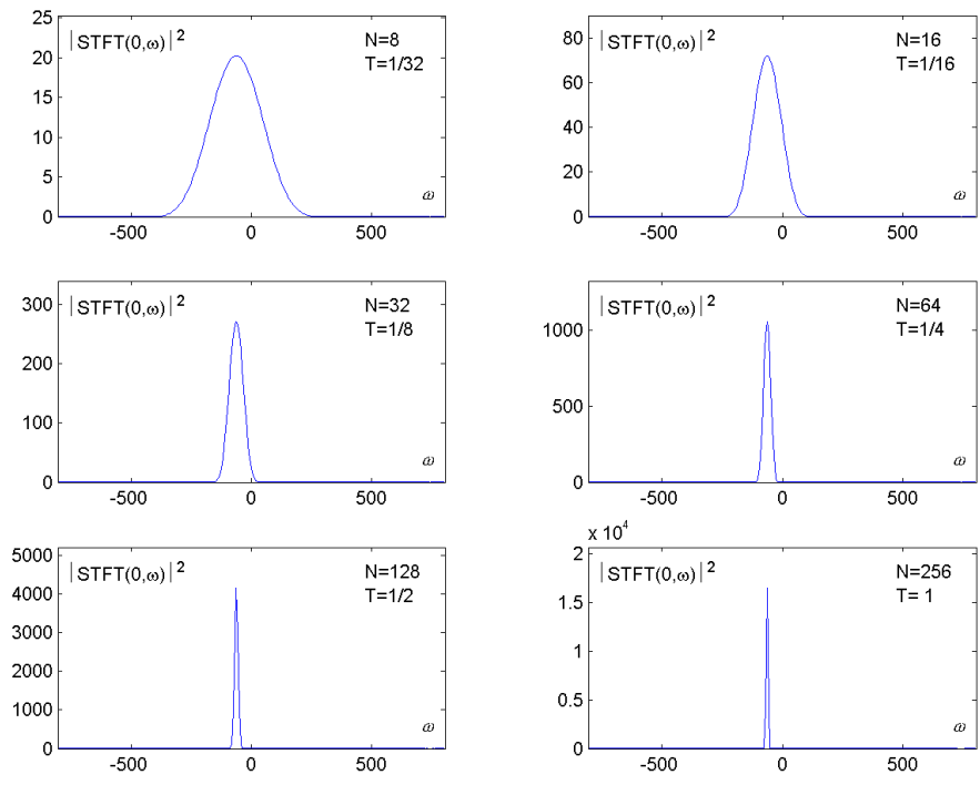
Figure 5: The spectrogram of the signal x(t) , at the time instant t = 0 and for various window widths T . Note that N is the number of samples within window.
