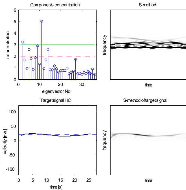
Figure 44: Signal 7: Time-frequency representation (top right), Concentration of the eigenvectors time-frequency representations (top left), Time-frequency representation of the detected target signal (bottom right), Highly concentrated time-frequency representation of the detected target signal (bottom left) and FFT estimation of the target velocity (dashed line)
