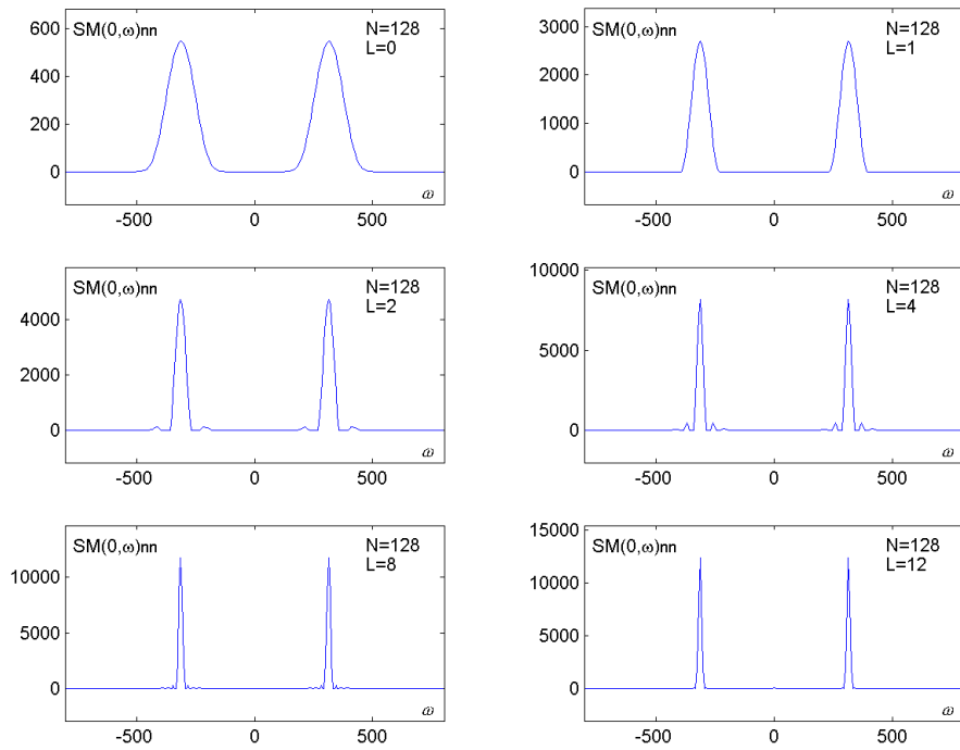
Figure 26: Only non-negative SM of two Linear Frequency Modulated Signal components x(t) , with fixed window width N = 128 , and L=0\dots 12 values
