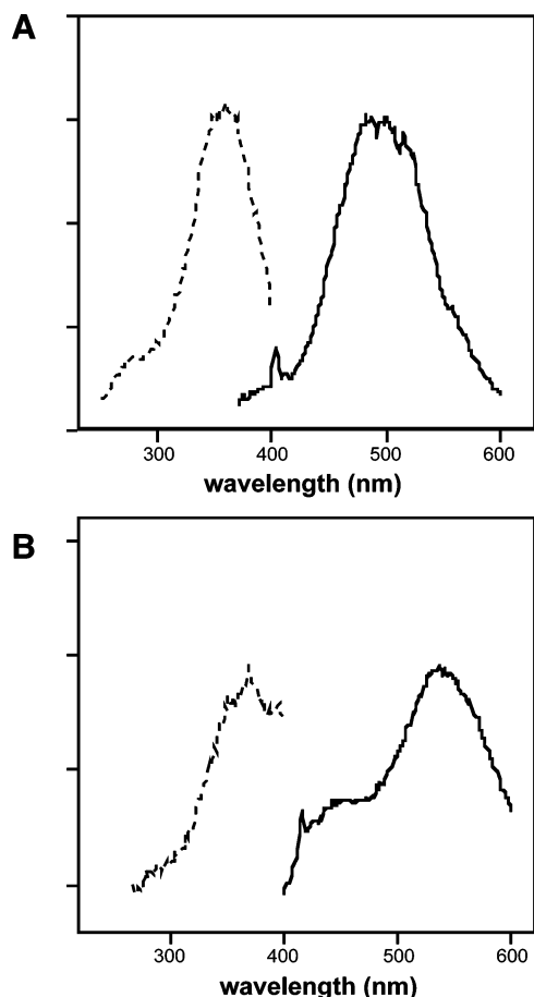
Figure 2. Excitation and emission spectra of 1 (A) and 2 (B) ( 2\ \mu\text{M} ) in methanol ( 25\ ^\circ\text{C} ). Excitation spectra are shown with dashed lines and were monitored at the emission maxima. Emission spectra are shown with solid lines and were measured with excitation at the long-wavelength absorption maxima.
