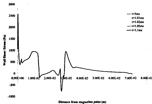
Fig. 14 Shear stress (upper)
