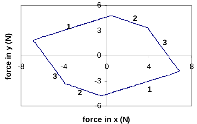
Figure 13: Force polytope for a 3-DOF planar robot.
