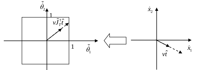
Figure 4: Joint speed limits and velocity vector expansion.
