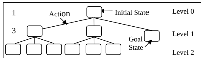
Figure 4: A simplistic planning tree for b = 3 and d = 2
