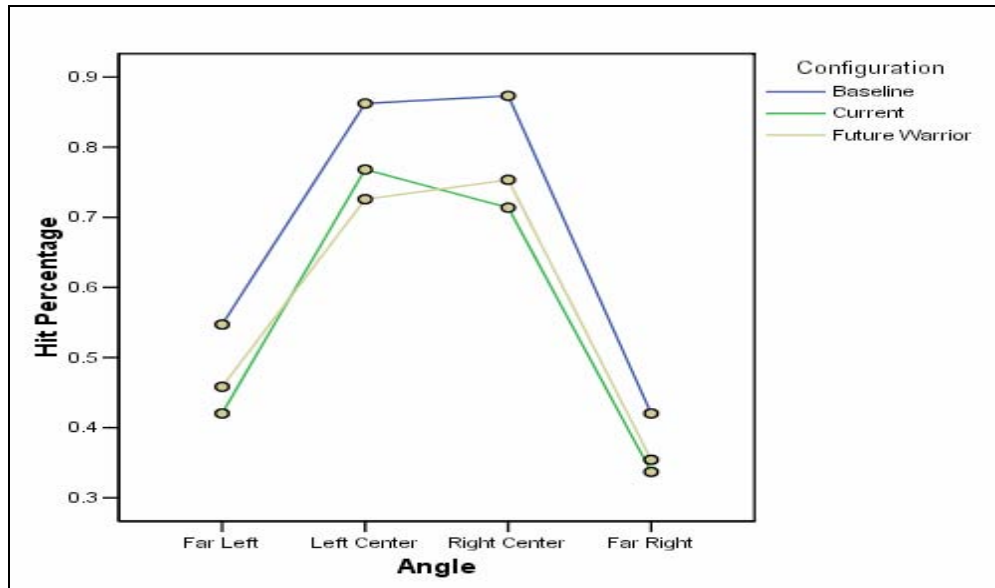
Figure 26. Mean hit percentages of four separate range sections in three encapsulation conditions.
