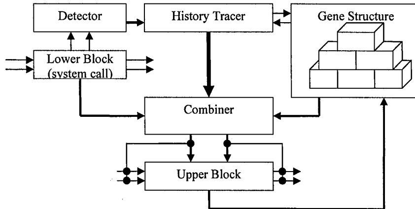
Fig. 2.14 Detection Algorithm for abnormal behavior
