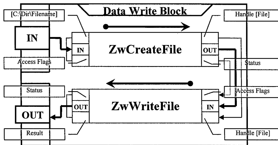
Fig. 2.2 GSR Building Block Internal Structure
