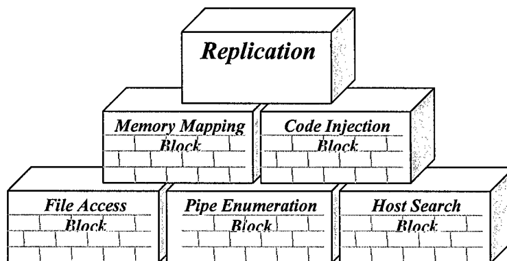
Fig. 2.11 Final replication behavior structure of a virus with networking capabilities
