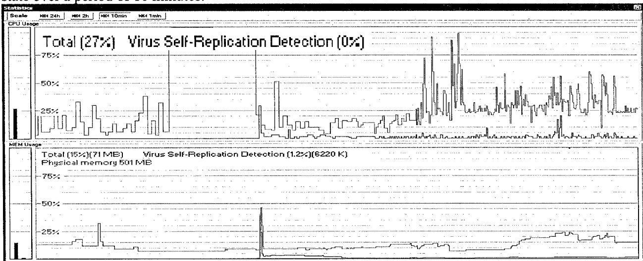
Fig. 2.12 CPU and Memory overhead versus total load, 10 minutes period
