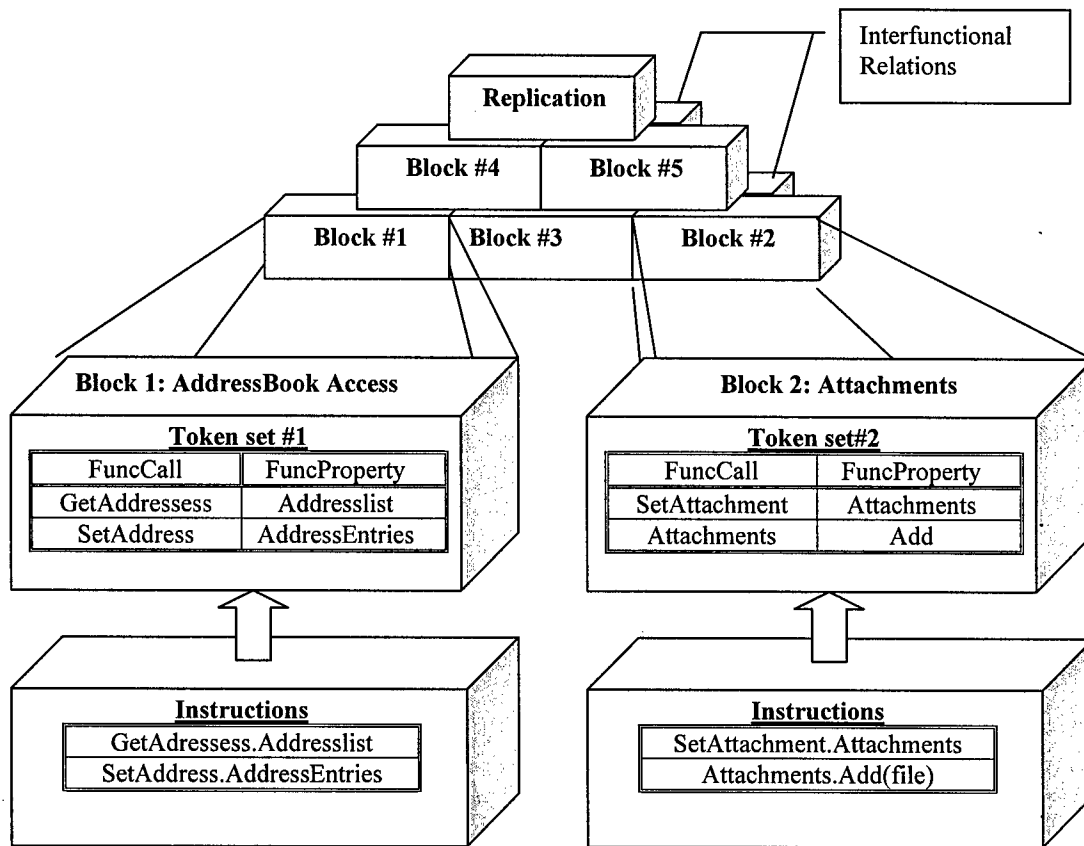
Fig.1.3. Evolution of the code. From instructions to the top of the pyramid.
