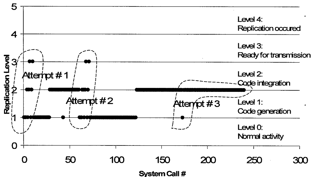
Fig. 2.9 Sample legitimate code activity graph 240 points, (3 attempts)
