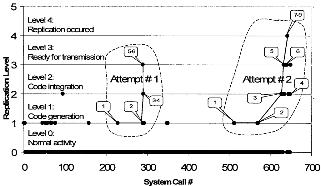
Fig. 2.7 Sample Virus Replication Data (648 points, 2 attempts)
