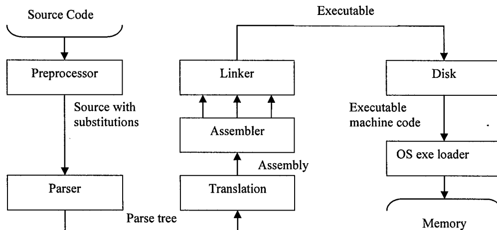
Fig.1.1 The compilation process
