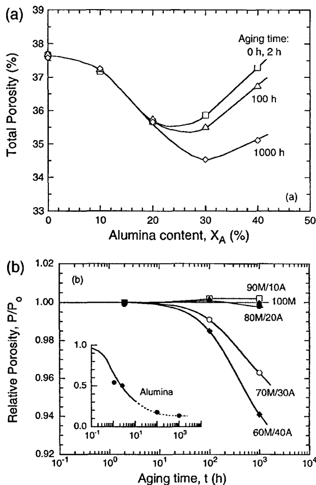
Fig. 2. (a) Effects of composition and aging time on compact porosity. The data for 0 h and 2 h are virtually identical to one another and are indistinguishable on the graph. (b) Results in (a), normalized by the initial (green) porosity at the same composition. The solid line for alumina in the inset was obtained by dilatometry; the symbols are based on the Archimedes measurements, and all other lines are simply curve fits through the discrete data points.
