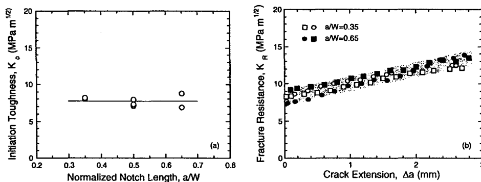
Figure 3. Effects of notch length on (a) the initiation fracture toughness and (b) the fracture resistance curve.
