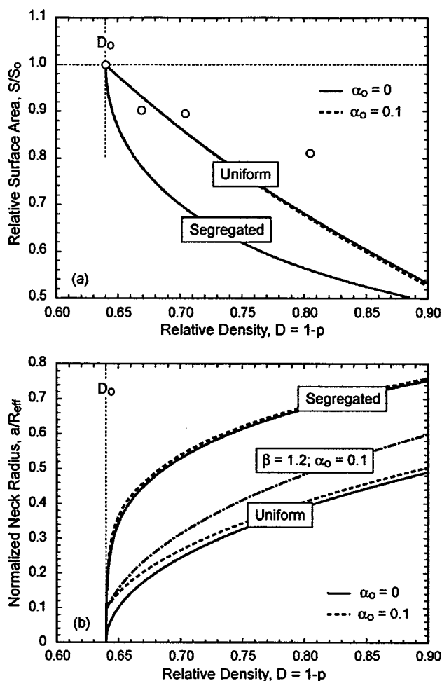
Fig. 6. Effects of precursor-derived alumina on (a) normalized specific surface area and (b) neck size. Details of the model predictions are given in the Appendix A. (Uncertainty in each measurement in (a) is less than the symbol size.)
