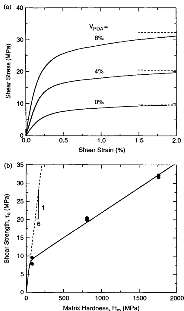
Fig. 10. Related effects of precursor-derived alumina (PDA) concentration and matrix hardness on composite shear properties: (a) stress-strain response and (b) shear strength. Dashed lines in (a) denote limit stress values at larger strains. Also shown in (b) is the expected trend for a ductile matrix composite (dashed line), subject to the Tresca yield criterion.
