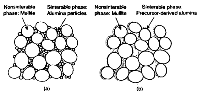
Fig. 1. Schematics showing the two matrix topologies produced by (a) mullite/alumina particle mixtures and (b) mullite particles bonded by precursor-derived alumina.
