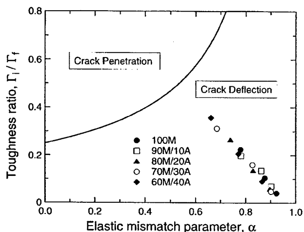
Fig. 1. Conditions for crack deflection at a fiber-matrix interface (solid line). Experimental measurements from this study are superimposed (symbols). The latter assume a toughness ratio \omega = \Gamma_i/\Gamma_m = 1 and fiber properties \Gamma_f = 15 \text{ J/m}^2 and E_f = 260 \text{ GPa} .
