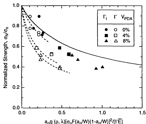
Fig. 11. Variation in notched strength with normalized notch length. Solid line is prediction of Eq. (9). Open symbols are experimental values, calculated using the total measured fracture energy; solid symbols are experimental values, calculated using the fracture energy without the pullout contribution.
