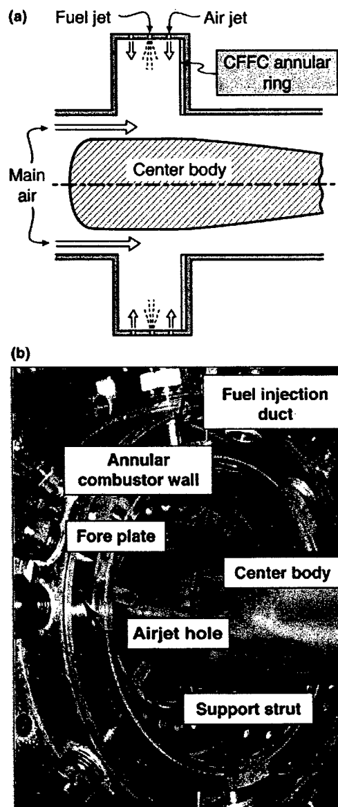
Fig. 2. (a) Schematic of longitudinal cross-section of ultra-compact combustor rig. (b) The combustor rig, disassembled to reveal the internal parts of the combustion chamber. (For scale, the inner radius of the combustor cavity is 59 mm.)
