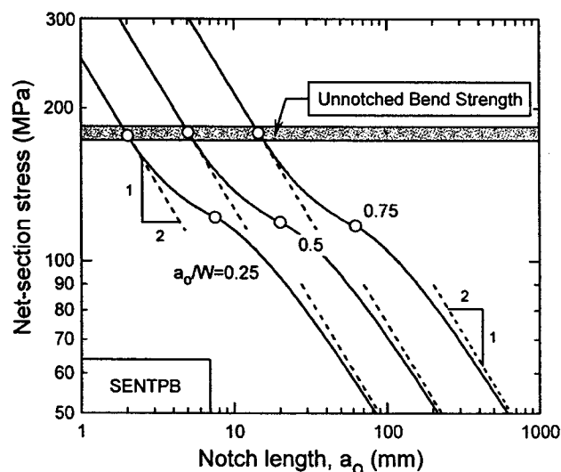
Fig. 8. Effects of a_0/W on notched strength of SENTPB specimen. The open circles show the behavioral transitions. For the transition II \rightarrow III (top row of circles), the critical notch length is given by Eq. (8); for the transition III \rightarrow IV (lower row of circles), it is given by Eq. (11).
