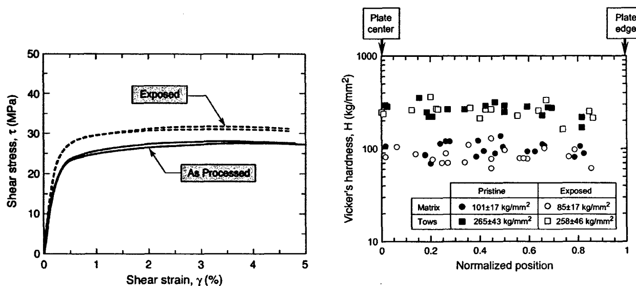
Fig. 10. Variation in hardness across plate thickness. Inset summarizes average values and standard deviations.
