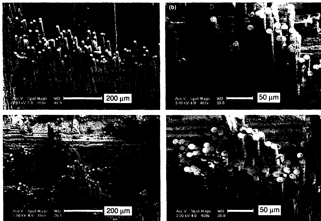
Fig. 8. Fracture surfaces of (a, b) pristine (as-processed) material and (c, d) after exposure in the combustor (ring #2).
