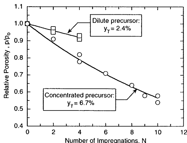
Fig. 4. Reduction in porosity following precursor impregnation and pyrolysis. Solid lines are fits of Eq. (2) to the experimental data.
