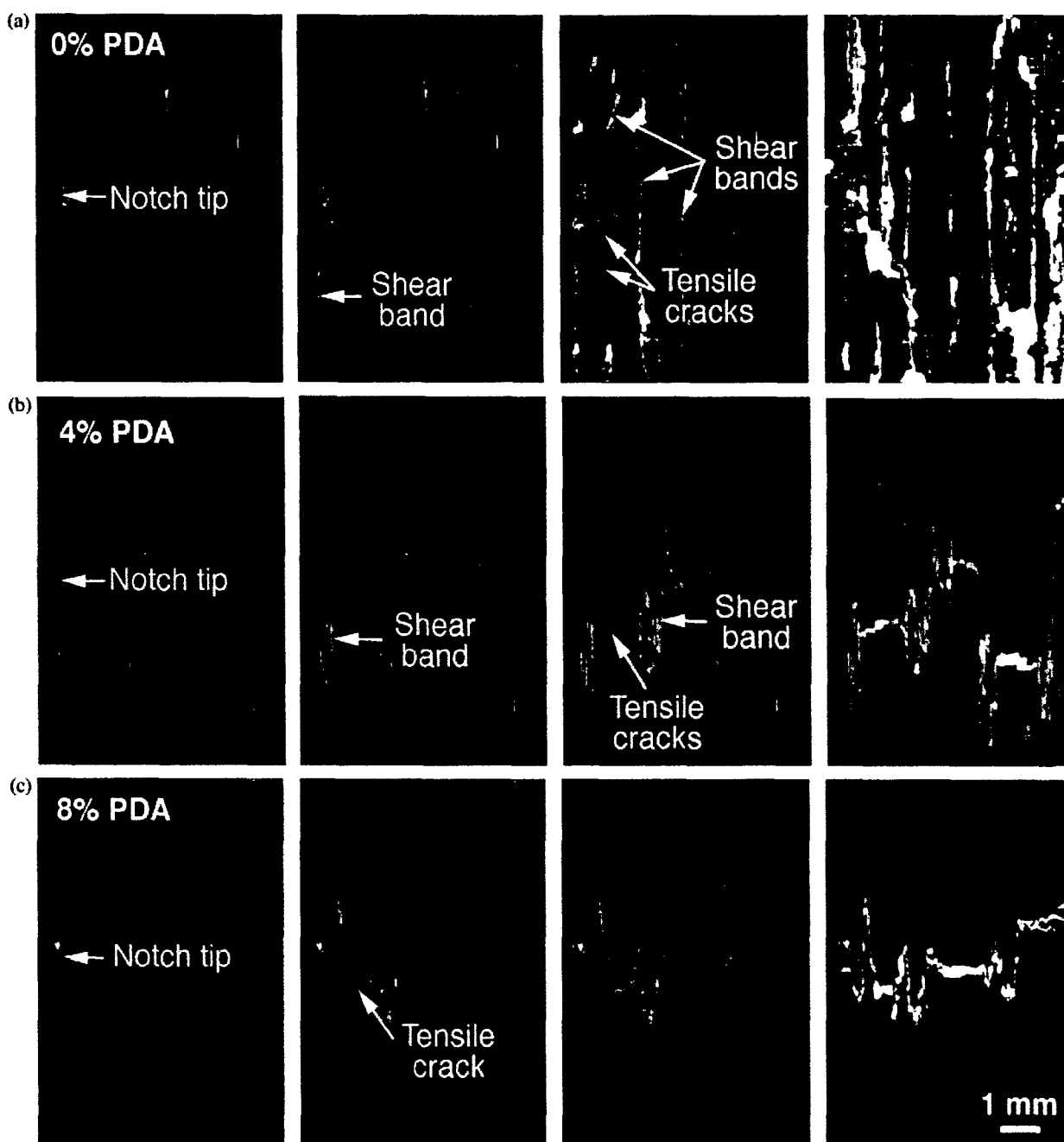
Fig. 6. Progression of damage in edge-notched tensile specimens: (a) V_{\text{PDA}} = 0 , (b) V_{\text{PDA}} = 4 , (c) V_{\text{PDA}} = 8 . In each sequence, the first picture represents the pristine (unloaded) specimen. The subsequent images are at progressively increasing displacements, indicated in Fig. 7. PDA, precursor-derived alumina.
