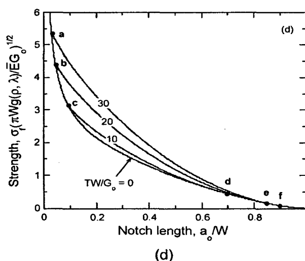
Fig. 3. Effects of tearing modulus on crack stability and strength for SENB.
