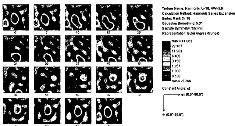
Fig. 26 (a) crack morphology and grain structure. (b) ODF of the recrystallized region ("A" in (a)), and (c) ODF of the unrecrystallized region ("B" in (a)) in the 2099 Al alloy.
