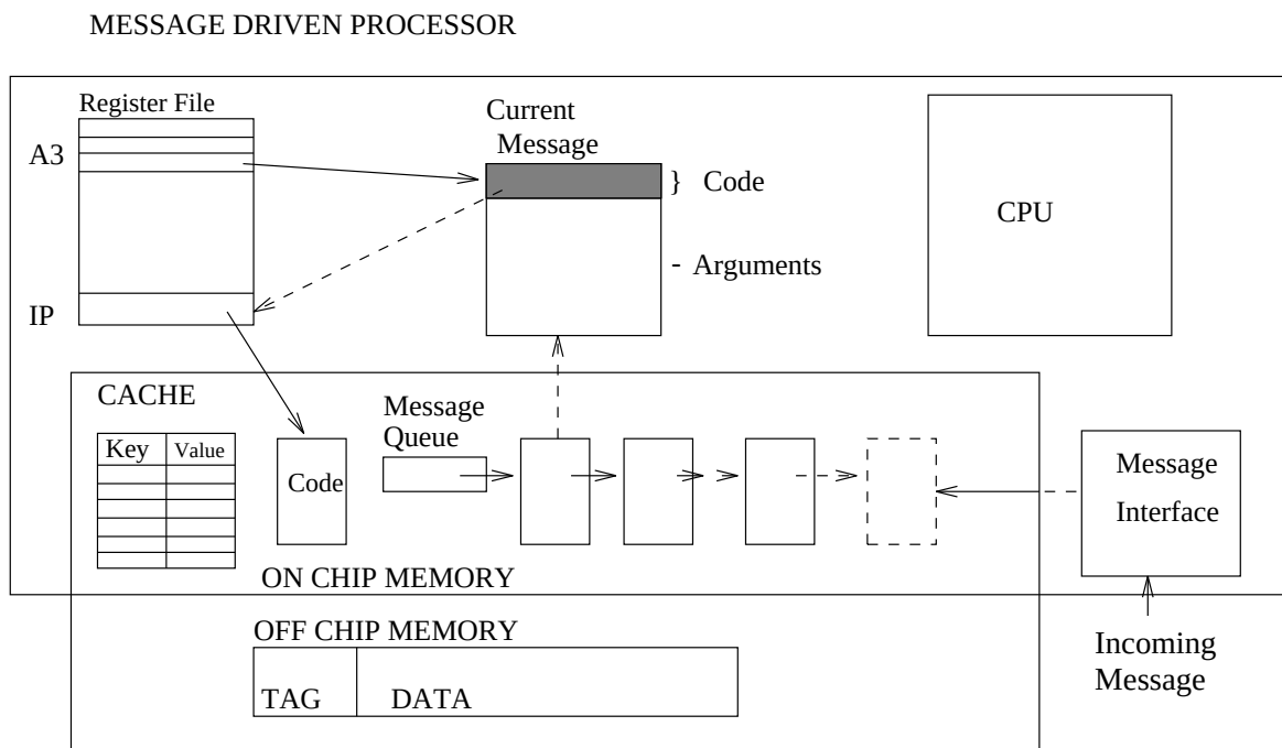
Figure 3.1: An Abstract View of the J-Machine
