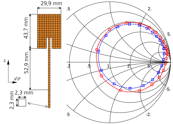
Fig. 4: Input impedance of a direct fed z -oriented microstrip antenna [5]. f_0=2.2\text{-}2.4 GHz (clockwise), \rho_0=30 mm, d_1=\rho_1-\rho_0=0.787 mm, \epsilon_{r1}=2.33 . Simulation ( \circ ), measurement ( \square ).
