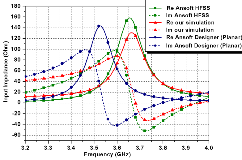
Fig.6: Input impedance of phi-polarized patch r_1=60 mm, r_0=58.42 mm, \epsilon_{r1}=2.52 quasi-rectangular \phi -polarized patch with sizes of w_\phi=25 mm, w_\theta=40 mm.
