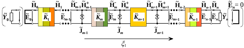
Fig. 2: Full-wave equivalent representation of a conformal multilayer structure, where \zeta_1 is the first of the curvilinear coordinates.
