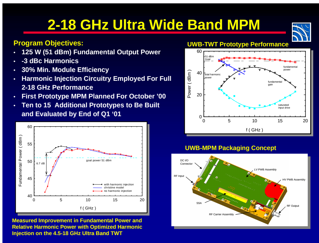
Performance of Northrop Grumman's Ultra-Wide Band MPM (Figure 20)
