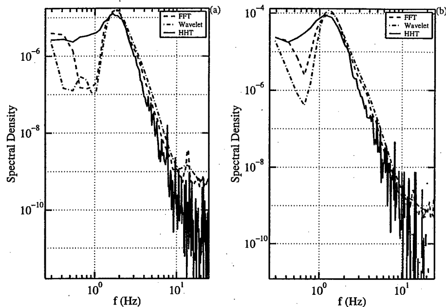
Figure 10.5: Spectra of wind-generated waves. The average wind speed is (a) 2 \text{ m s}^{-1} and (b) 5 \text{ m s}^{-1} .
