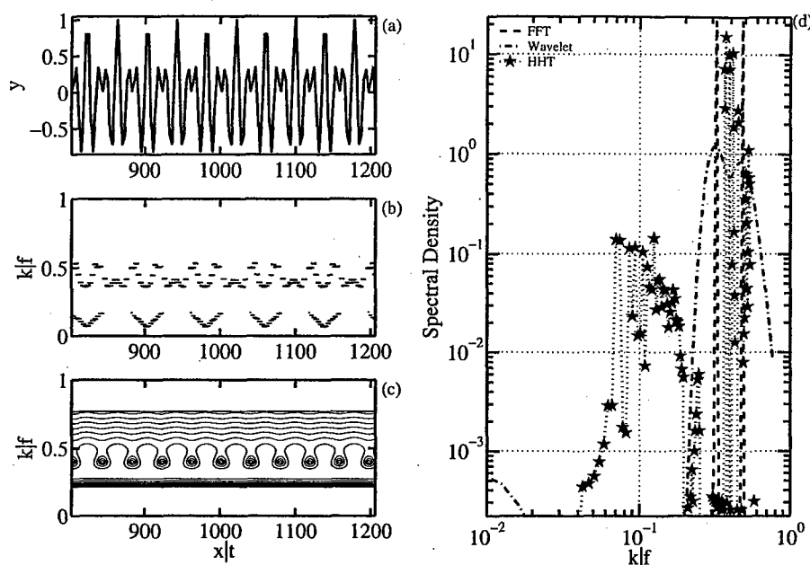
Figure 10.10: Same as Fig. 10.8, but the carrier period is 5\Delta t , and the modulation period is 25\Delta t , where \Delta t is the sampling time interval.
