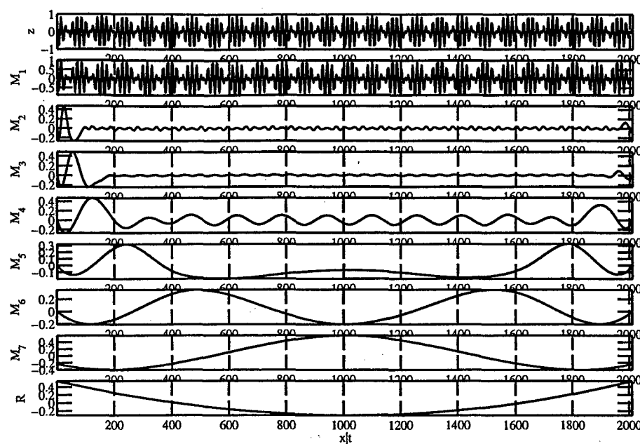
Figure 10.9: EMD processing of the signal shown in Fig. 10.8(a). The top panel is the original signal, M_1 to M_7 , are the modes and R is the remainder.
