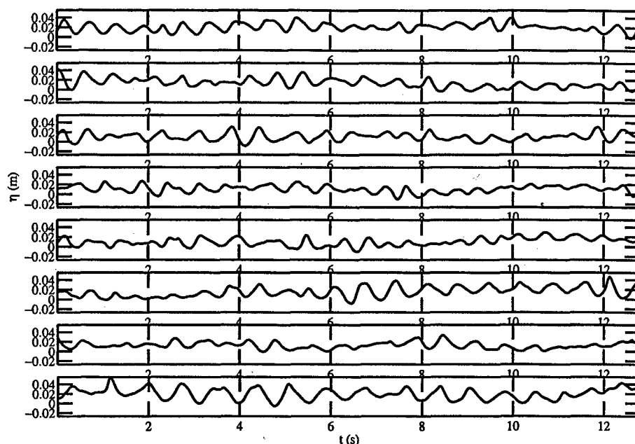
Figure 10.4: Examples of the time series of wind-generated waves used for spectral comparison. The average wind speed is about 5 \text{ m s}^{-1} . The data are measured by a fast response wire gauge sampled at 50 Hz.
