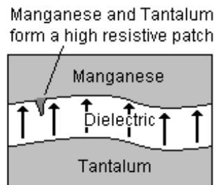
Figure 7 - Cross section of degraded Manganese Dioxide
