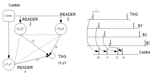
Fig. 1. Localization system with 3 readers and one tag
