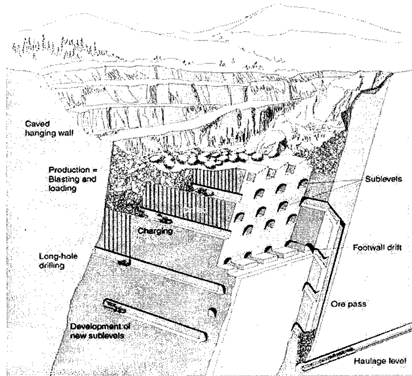
Figure 1.1. An example of sublevel caving (Altas Copco, 2005).
