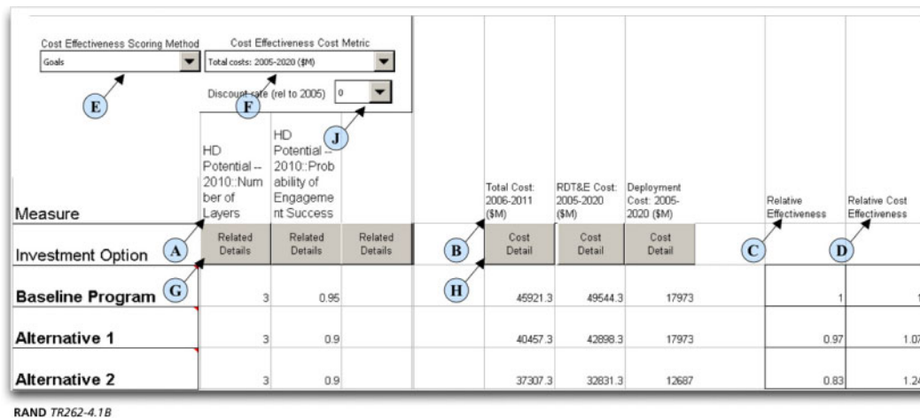
Figure 4.1b Right Side of Summary Sheet
