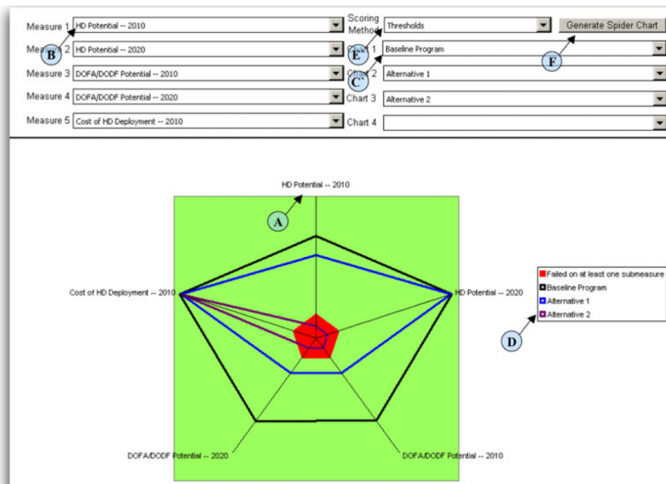
Figure 4.5 Multi-Measure Spider Charts Sheet
