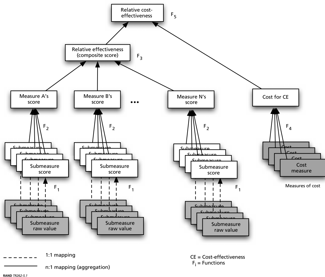
Figure 5.1 Generation of Scores, Effectiveness, and Cost-Effectiveness in PAT-MD (shaded items are inputs)
