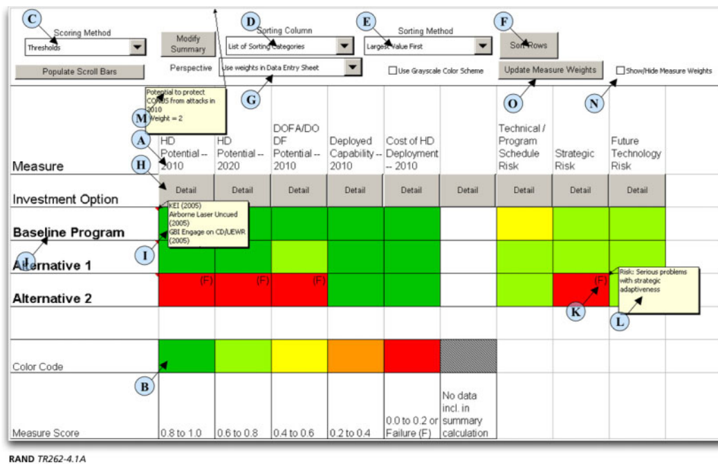
Figure 4.1a Left Side of Summary Sheet
