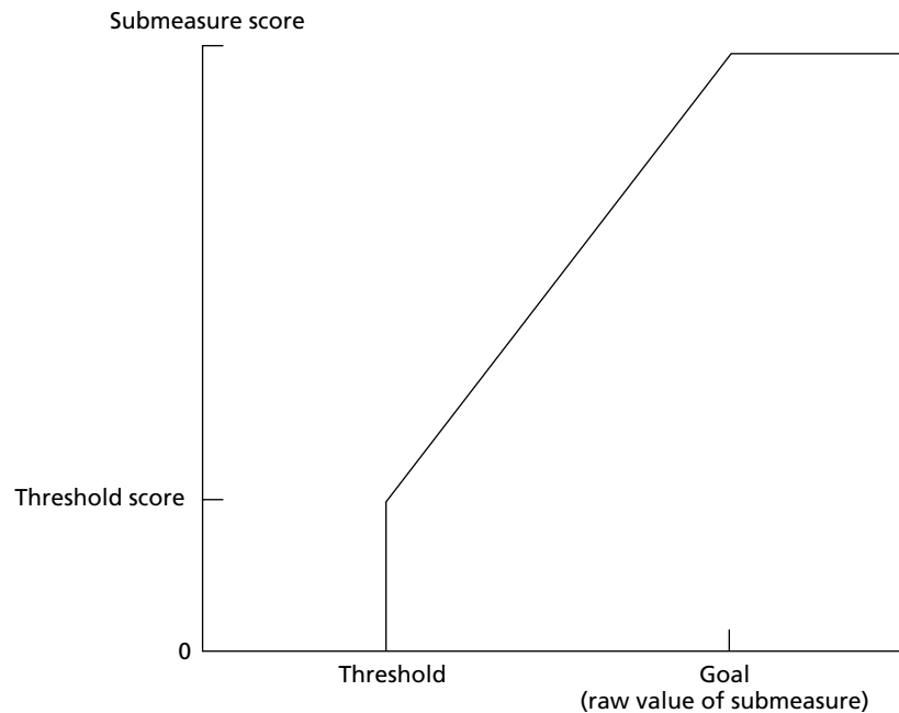
Figure 2.3 Mapping of Raw Submeasure Values into Scores
