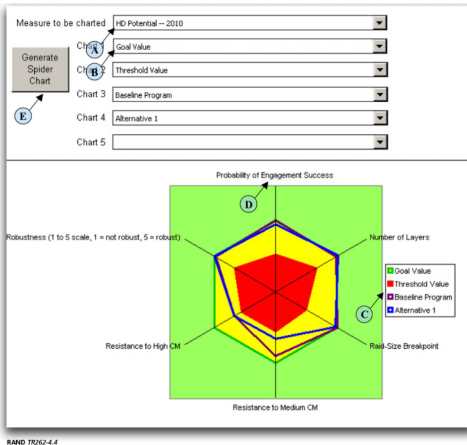
Figure 4.4 Spider Charts (Radar Charts) Sheet
