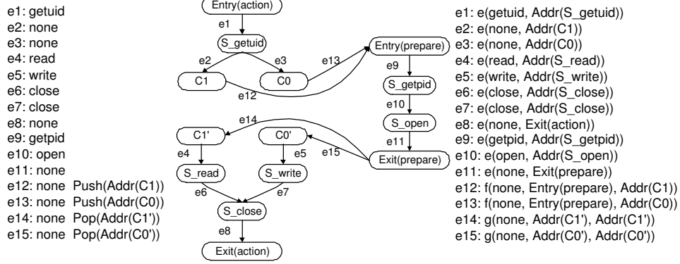
Figure 3. The PDA and VPStatic DPDA generated for the code example.
