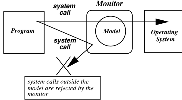
Figure 1. Architecture of a host-based intrusion detection system.
