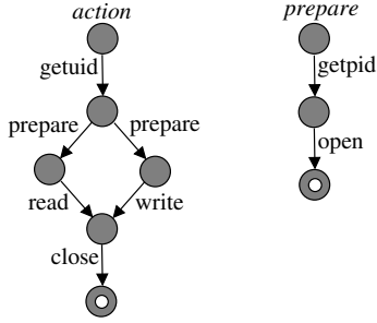
Figure 5. Local Dyck models.
