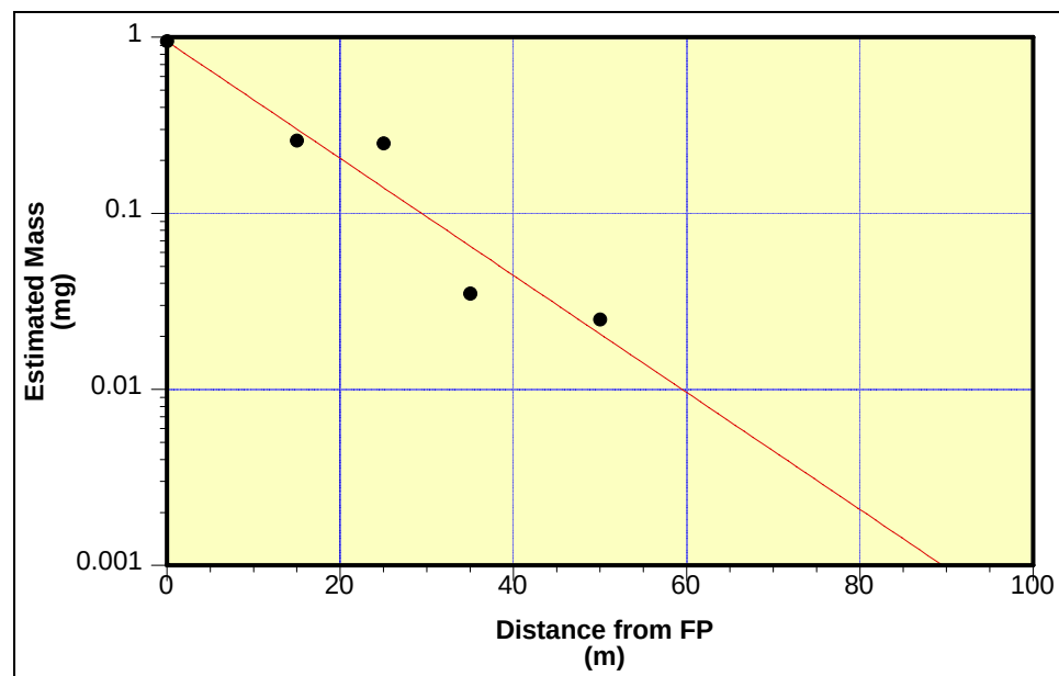
Figure 16. Exponential curve fit for FP residues (●): Case 2.
