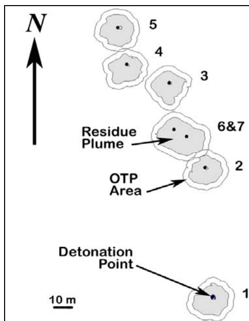
Figure 14. 60-mm M888 HE round detonation plumes: Sampled plumes.
