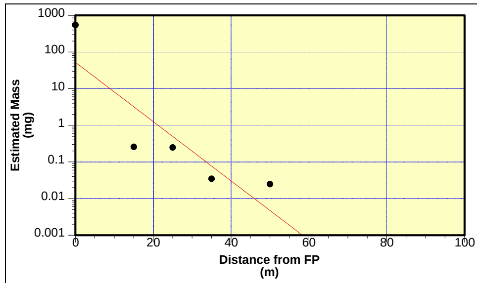
Figure 15. Exponential curve fit for FP residues (●): Case 1.
