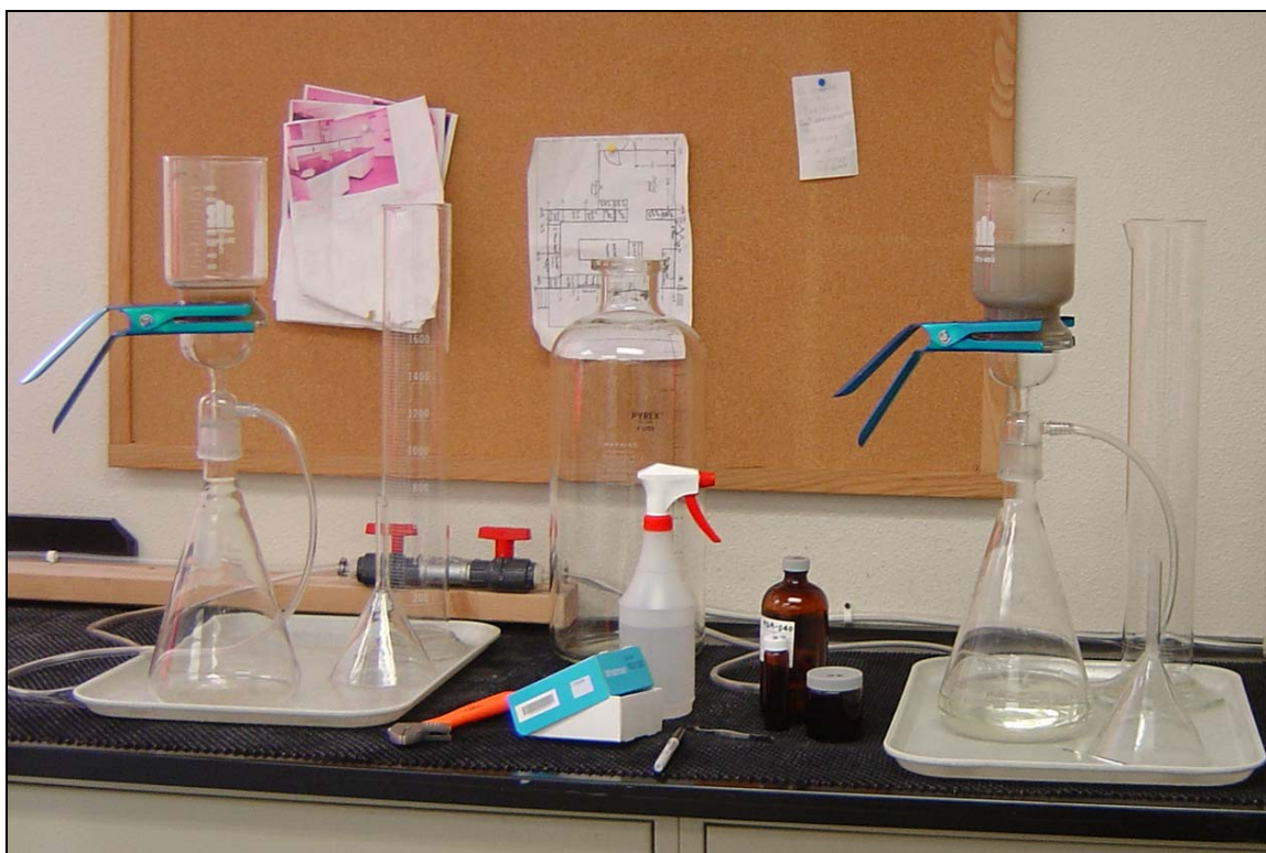
Figure 10. Sample filtration setup.
