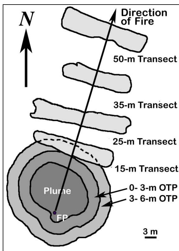
a. 60-mm mortar firing.
