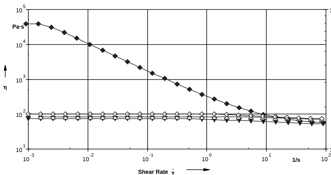
Figure 12. Viscosity of nanomaterials with respect to shear rate. \blacklozenge is 5% R202, \blacktriangledown is neat 977-3, \triangle is 5% 520H, and \diamond is 5% \text{Ph}_{12}\text{T}_{12} .
