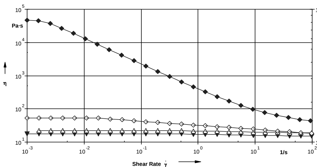
Figure 13. Viscosity of nanomaterials with respect to shear rate. \blacklozenge is 5% R202, \blacktriangledown is neat 977-3, \triangle is 5% 520H, and \diamond is 5% \text{Ph}_{12}\text{T}_{12} .
