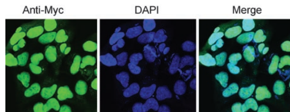
Fig. 2. Myc-tagged SUMO and sumoylated proteins mainly localized in the nucleus. After Myc-SUMO stably expressed HEK 293 Tet-On cells were induced with 2 \mu g/ml Dox for 48 h, cells were fixed with 3.7% formaldehyde and stained with anti-Myc primary antibody and FITC-conjugated secondary antibody. DAPI was used to stain nuclei.
