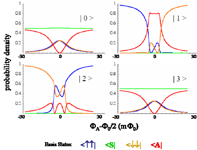
Fig. 13 Calculated wave functions near the double degeneracy point. Probability density for each of the four basis states is plotted for the states |0\rangle , |1\rangle , |2\rangle and |3\rangle .
