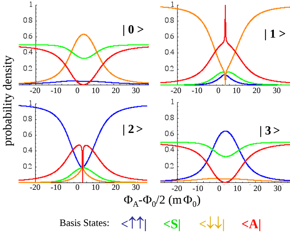
Fig. 10 Calculated wave functions near the intersecting degeneracy point. Probability density for each of the four basis states is plotted for the states |0\rangle , |1\rangle , |2\rangle and |3\rangle .
