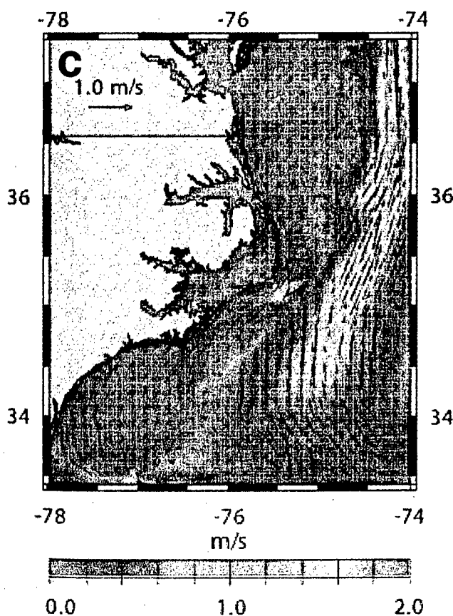
Figure 3. Predicted environmental conditions at landfall (16:00 UT 18 September 2003): a) The wind velocity computed by the Holland Model; b) The significant wave height from SWAN; c) The surface currents calculated by NCOM; and d) The water level anomaly calculated by NCOM (contour interval is 0.1 m).
