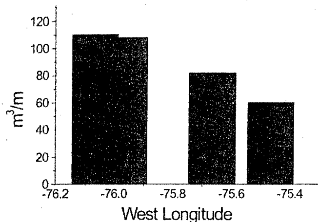
Figure 4. Potential erosion ( \text{m}^3 ) predicted by TRANS98 during Hurricane Isabel at the locations shown in Figure 1b. The distance from landfall is given in parentheses. The units are cubic meters of sand eroded per meter of coastline.
